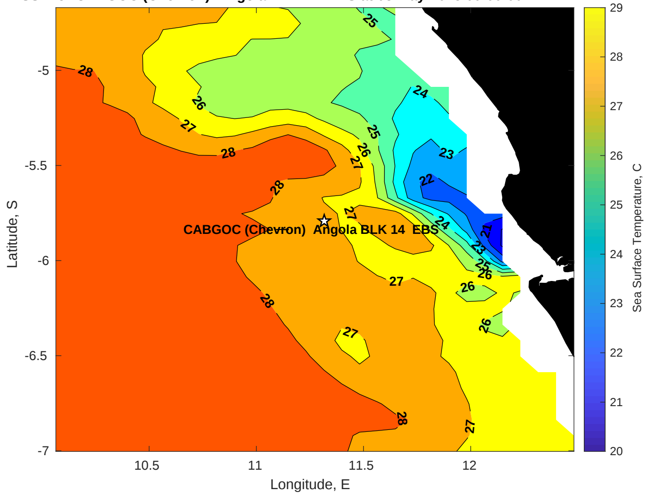
SST for CABGOC (Chevron) Angola BLK 14 EBS at 08-May-2025 00:00:00
