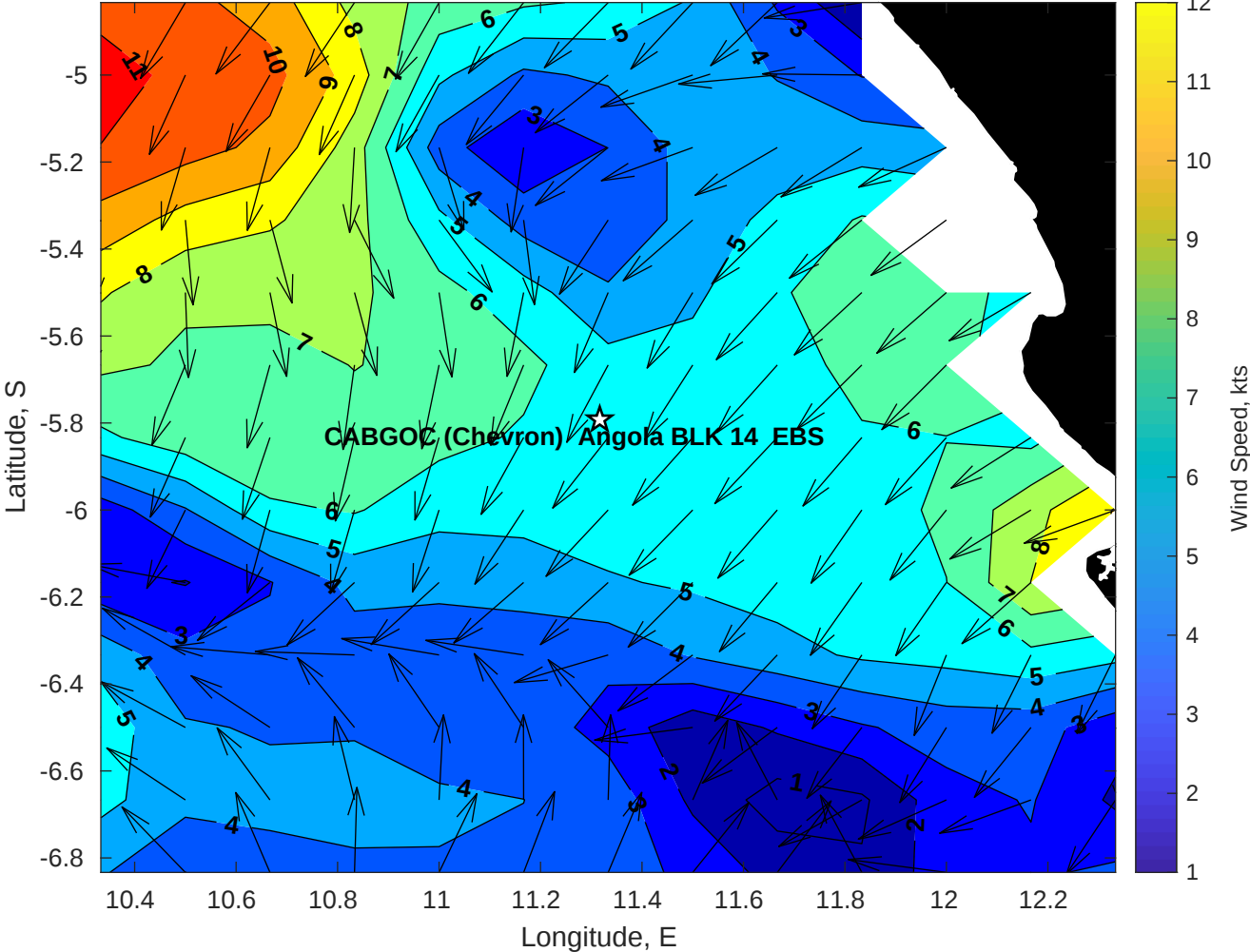
Winds (kts) for CABGOC (Chevron) Angola BLK 14 EBS at 09-May-2025 09:00:00
