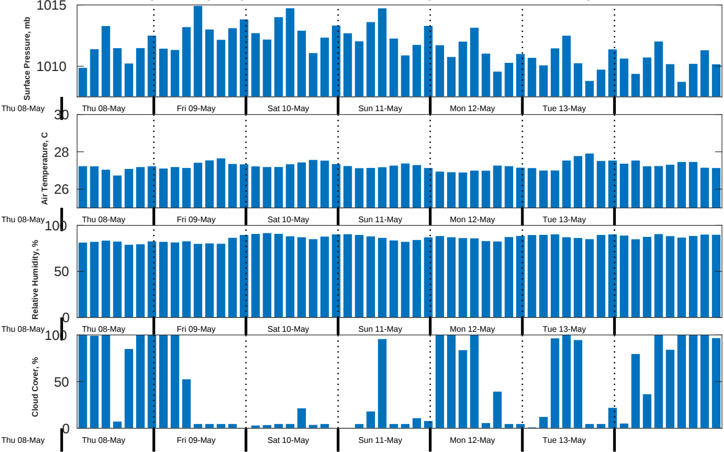
Met Forecast for CABGOC (Chevron) Angola BLK 14 EBS from 09-May-2025 00:00:00 to 16-May-2025 00:00:00
