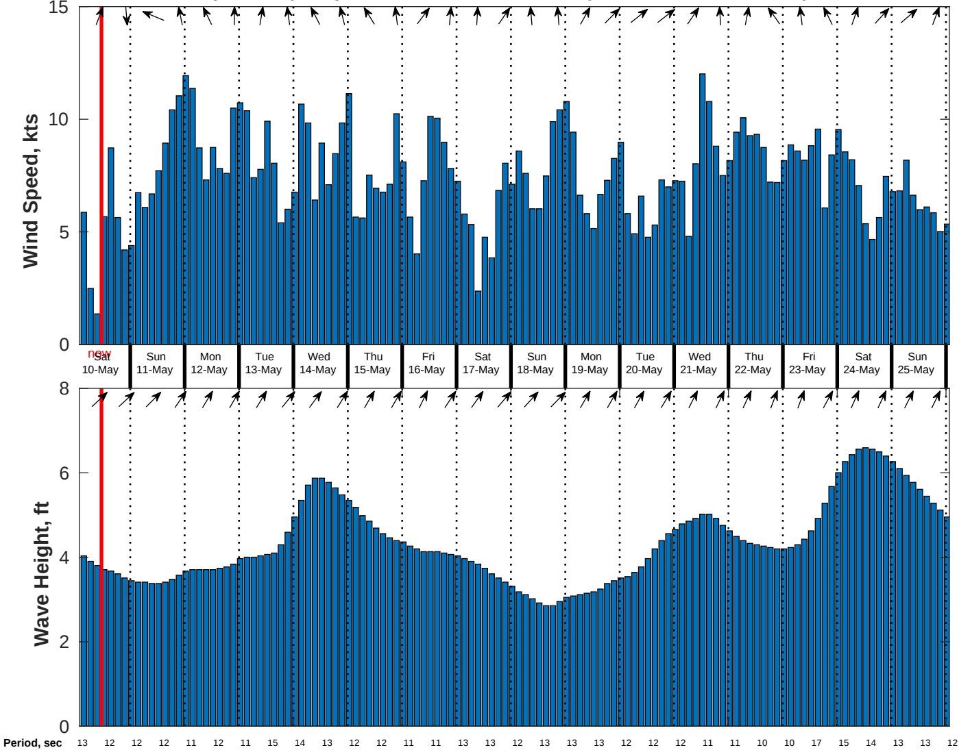
Wind & Wave Forecast for CABGOC (Chevron) Angola BLK 14 EBS from 09-May-2025 02:00:00 to 25-May-2025 02:00:00
