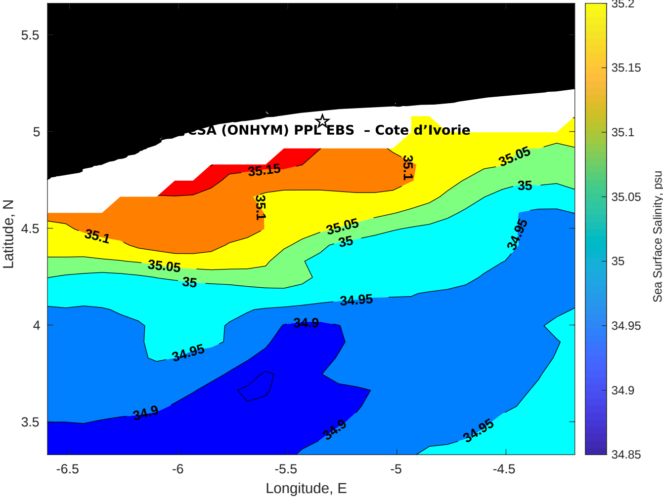
Surface Salinity for CSA (ONHYM) PPL EBS - Cote d'Ivoire at 08-May-2025 00:00:00
