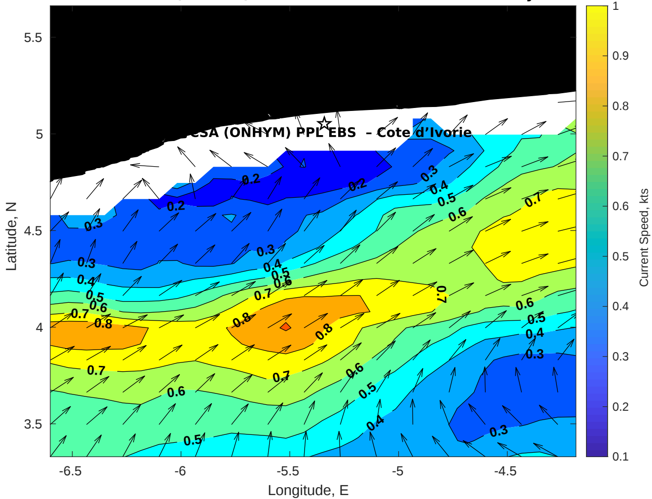
Surface Currents for CSA (ONHYM) PPL EBS - Cote d'Ivoire at 08-May-2025 00:00:00
