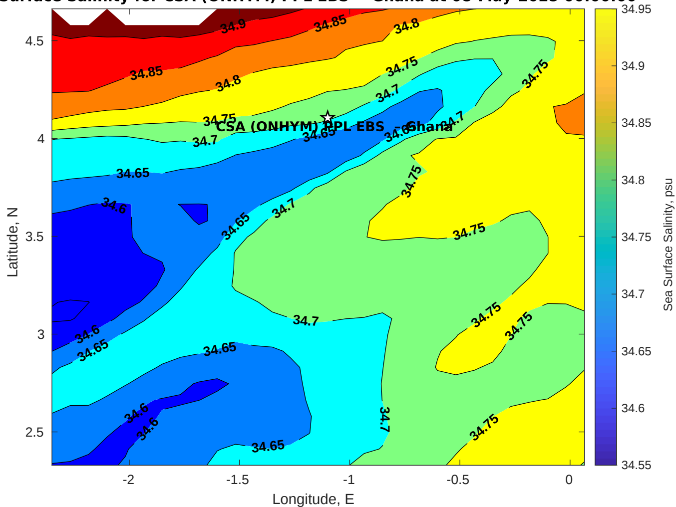
Surface Salinity for CSA (ONHYM) PPL EBS - Ghana at 08-May-2025 00:00:00
