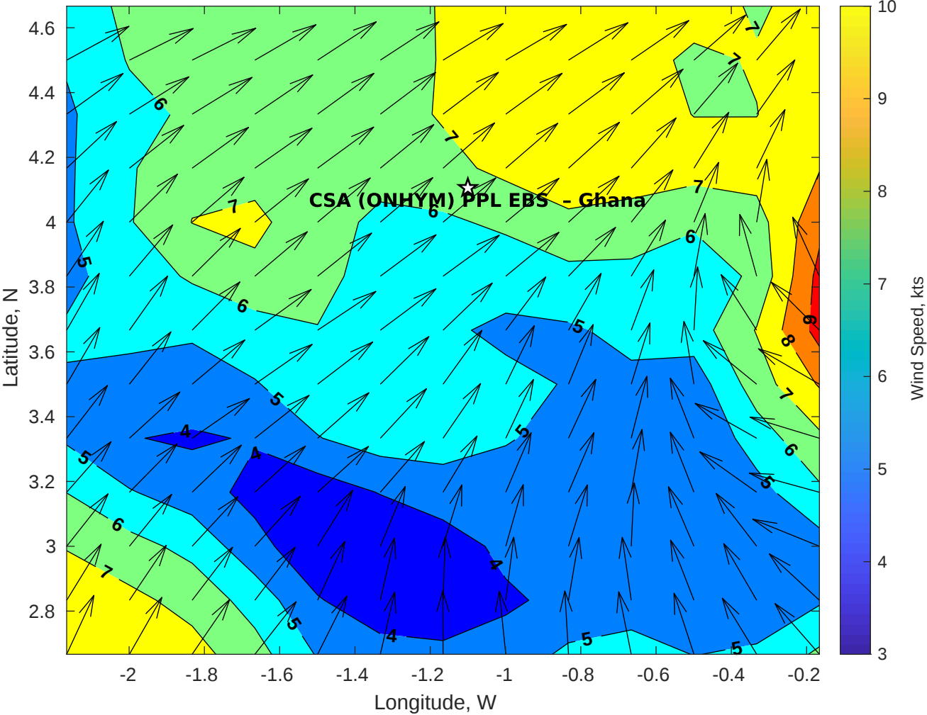
Winds (kts) for CSA (ONHYM) PPL EBS - Ghana at 09-May-2025 09:00:00
