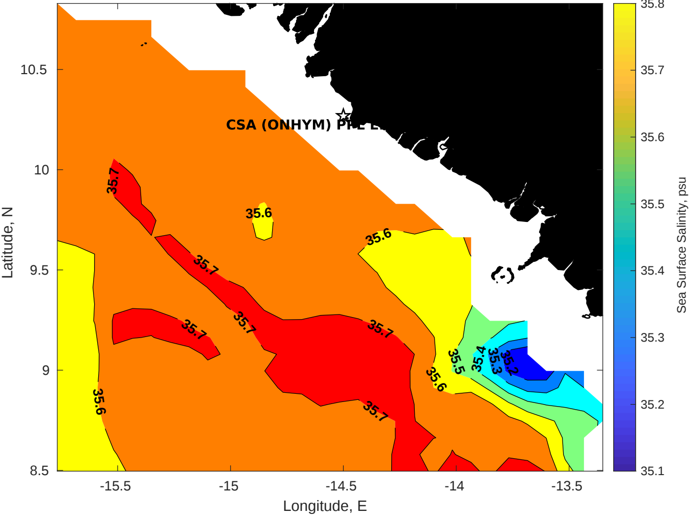
Surface Salinity for CSA (ONHYM) PPL EBS - Guinea at 08-May-2025 00:00:00
