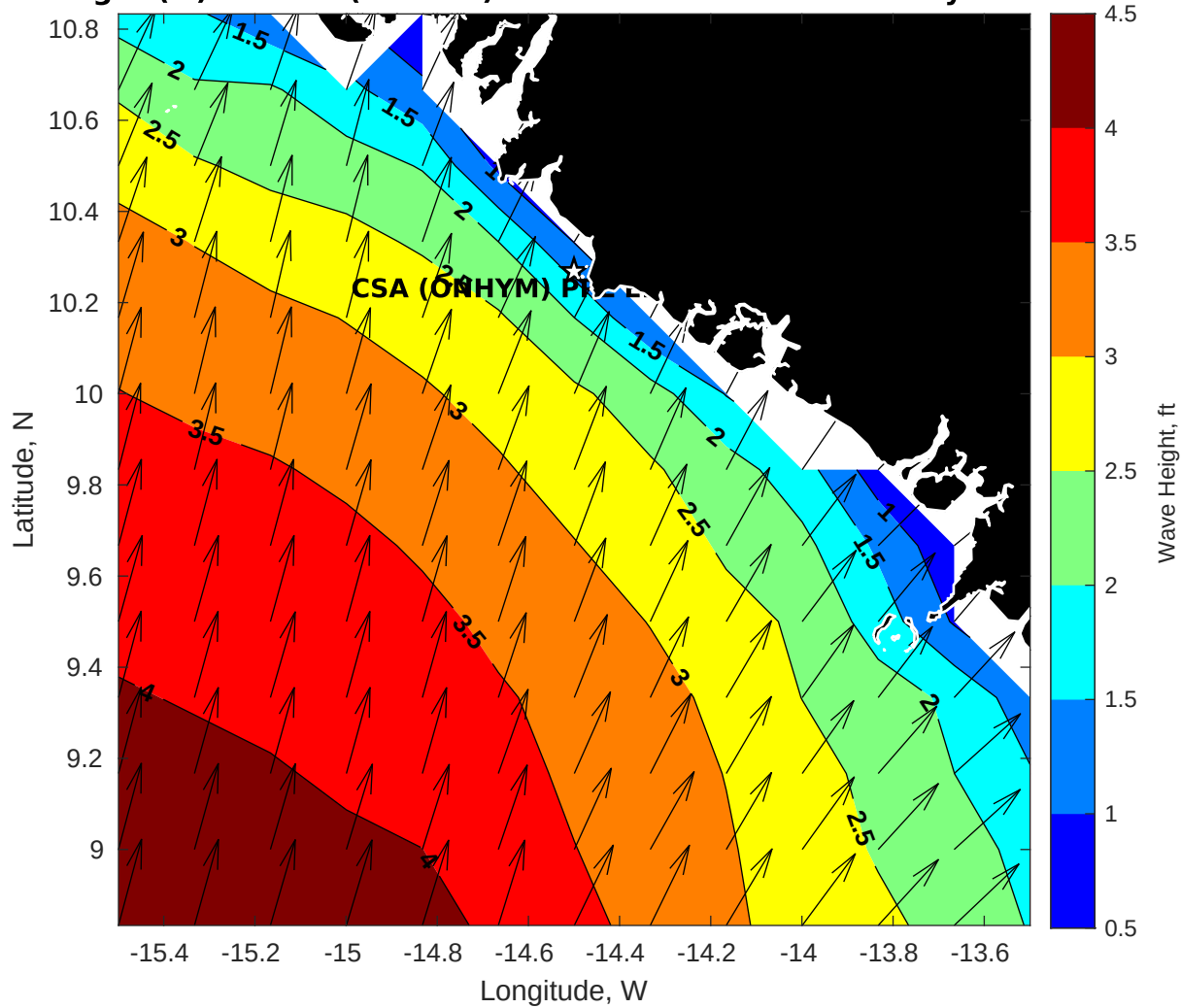
Wave Height (ft) for CSA (ONHYM) PPL EBS - Guinea at 09-May-2025 09:00:00
