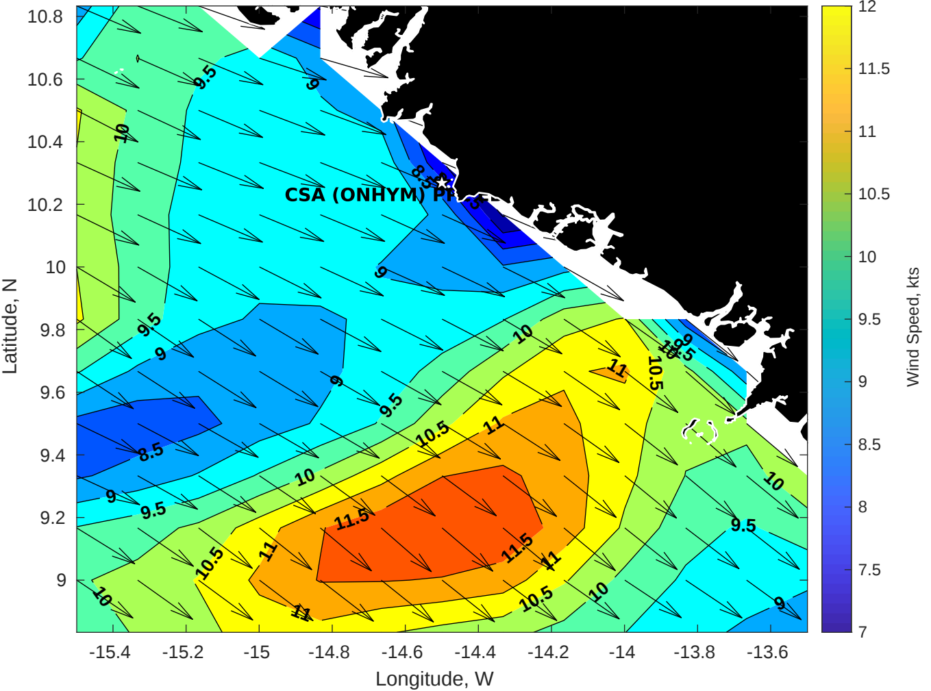
Winds (kts) for CSA (ONHYM) PPL EBS - Guinea at 09-May-2025 09:00:00
