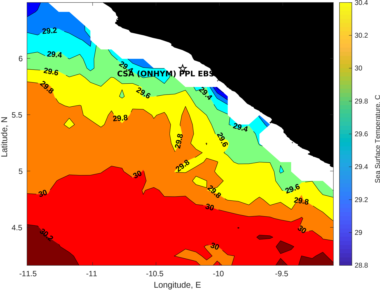
SST for CSA (ONHYM) PPL EBS - Liberia at 08-May-2025 00:00:00
