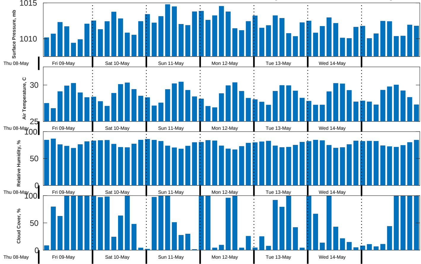
Met Forecast for CSA (ONHYM) PPL EBS - Liberia from 09-May-2025 00:00:00 to 16-May-2025 00:00:00
