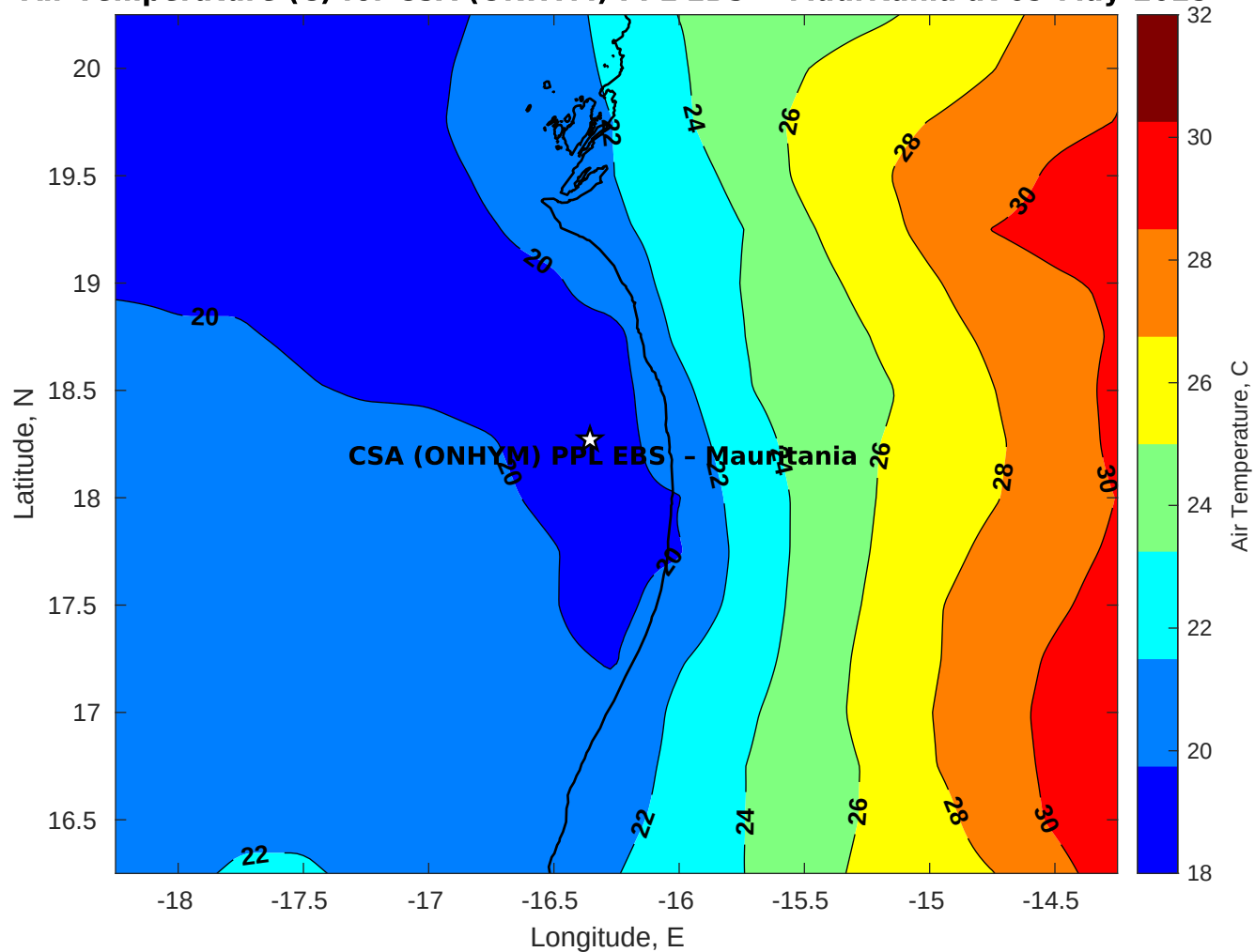
Air Temperature (C) for CSA (ONHYM) PPL EBS - Mauritania at 09-May-2025
