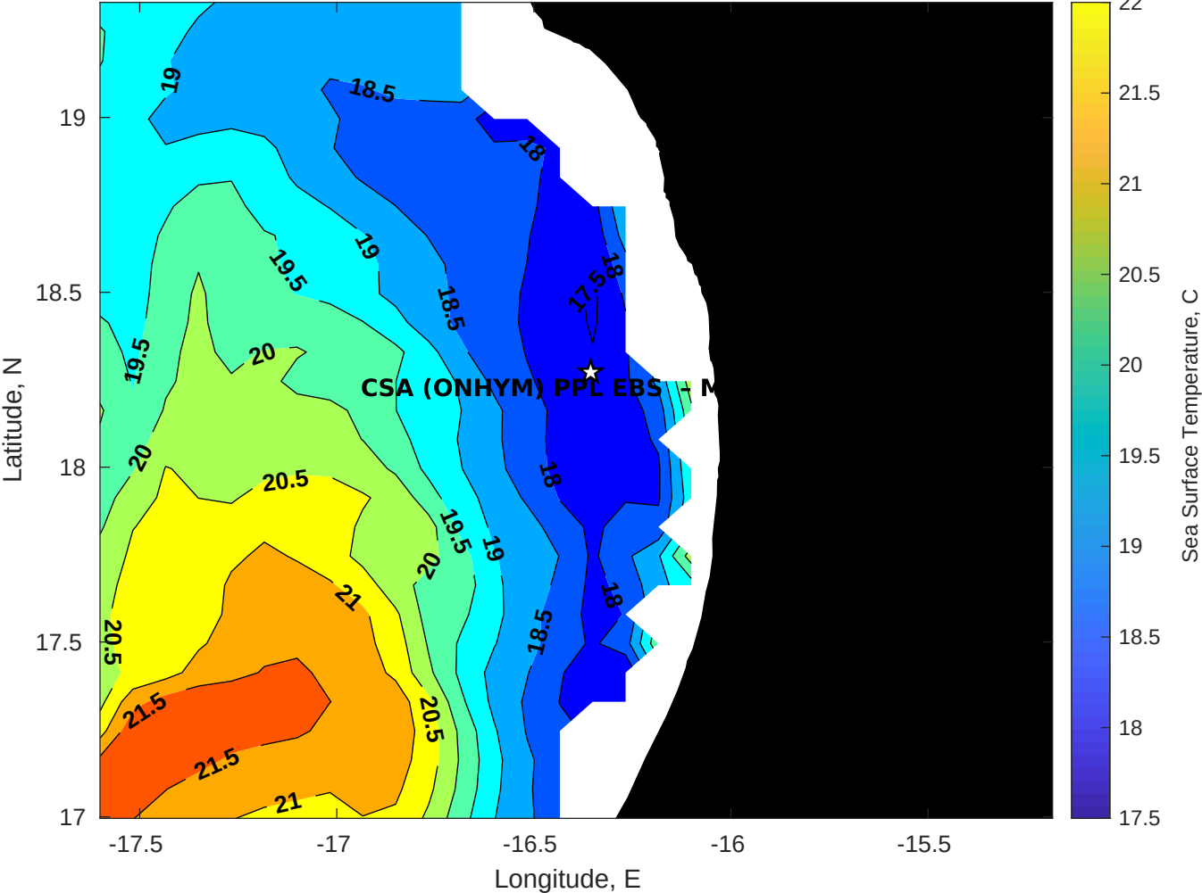
SST for CSA (ONHYM) PPL EBS - Mauritania at 08-May-2025 00:00:00
