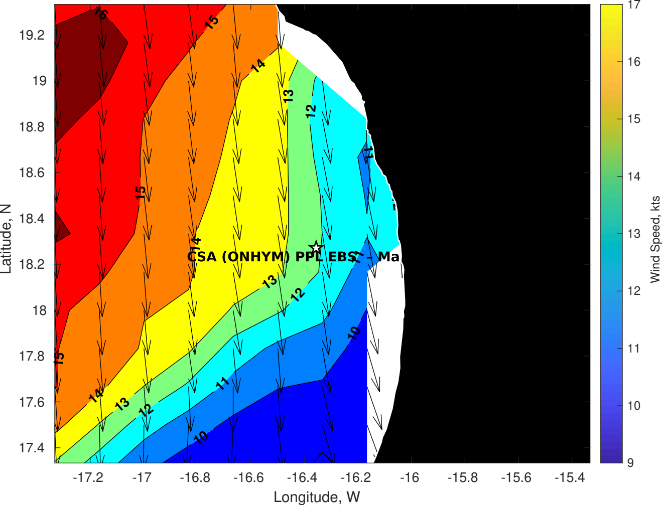
Winds (kts) for CSA (ONHYM) PPL EBS - Mauritania at 09-May-2025 09:00:00
