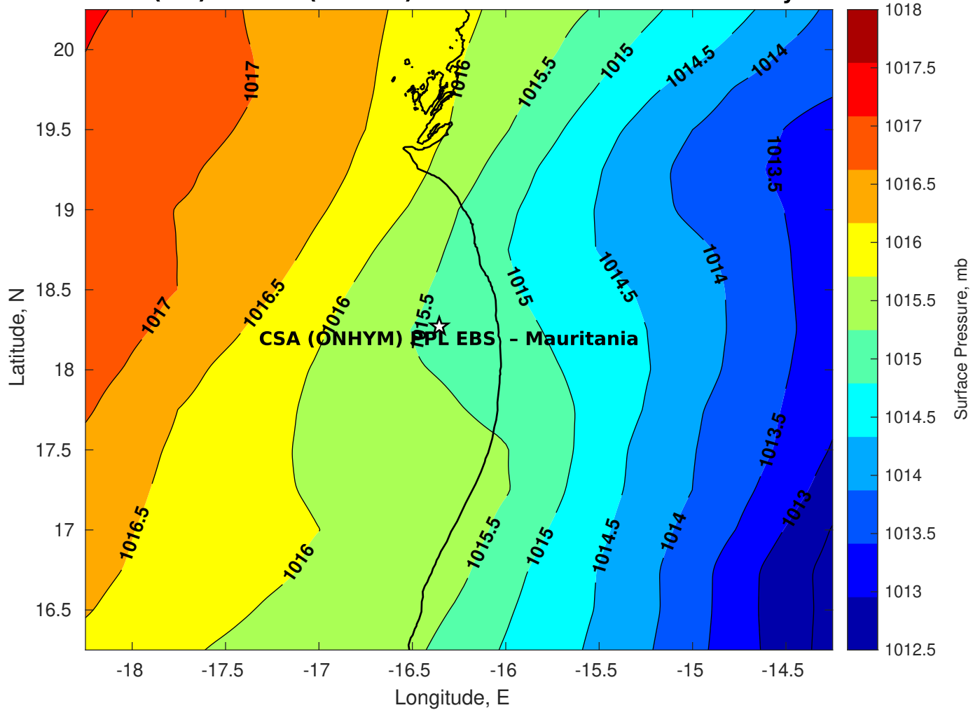
Surface Pressure (mb) for CSA (ONHYM) PPL EBS - Mauritania at 11-May-2025 00:00:00
