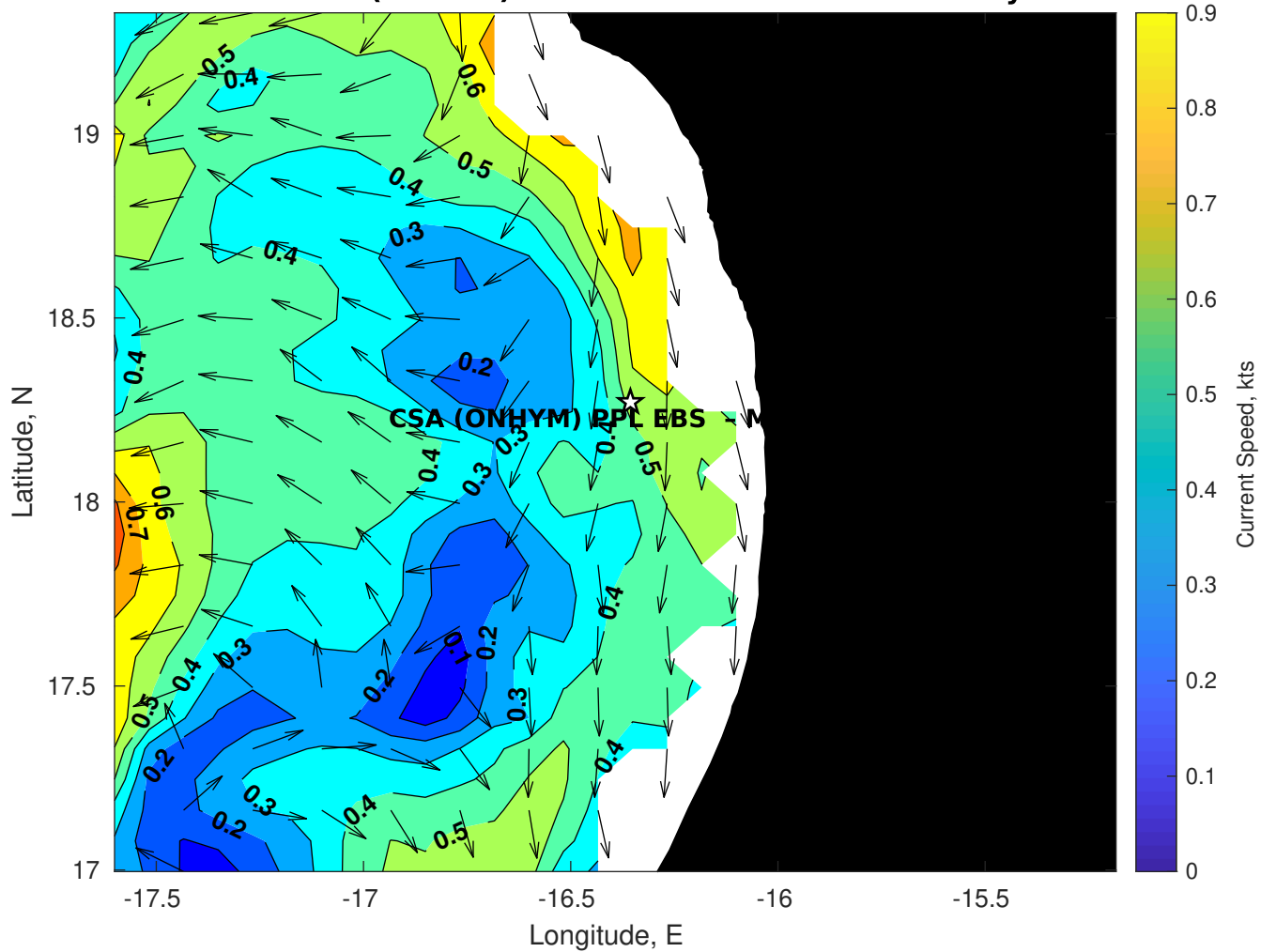
Surface Currents for CSA (ONHYM) PPL EBS - Mauritania at 08-May-2025 00:00:00
