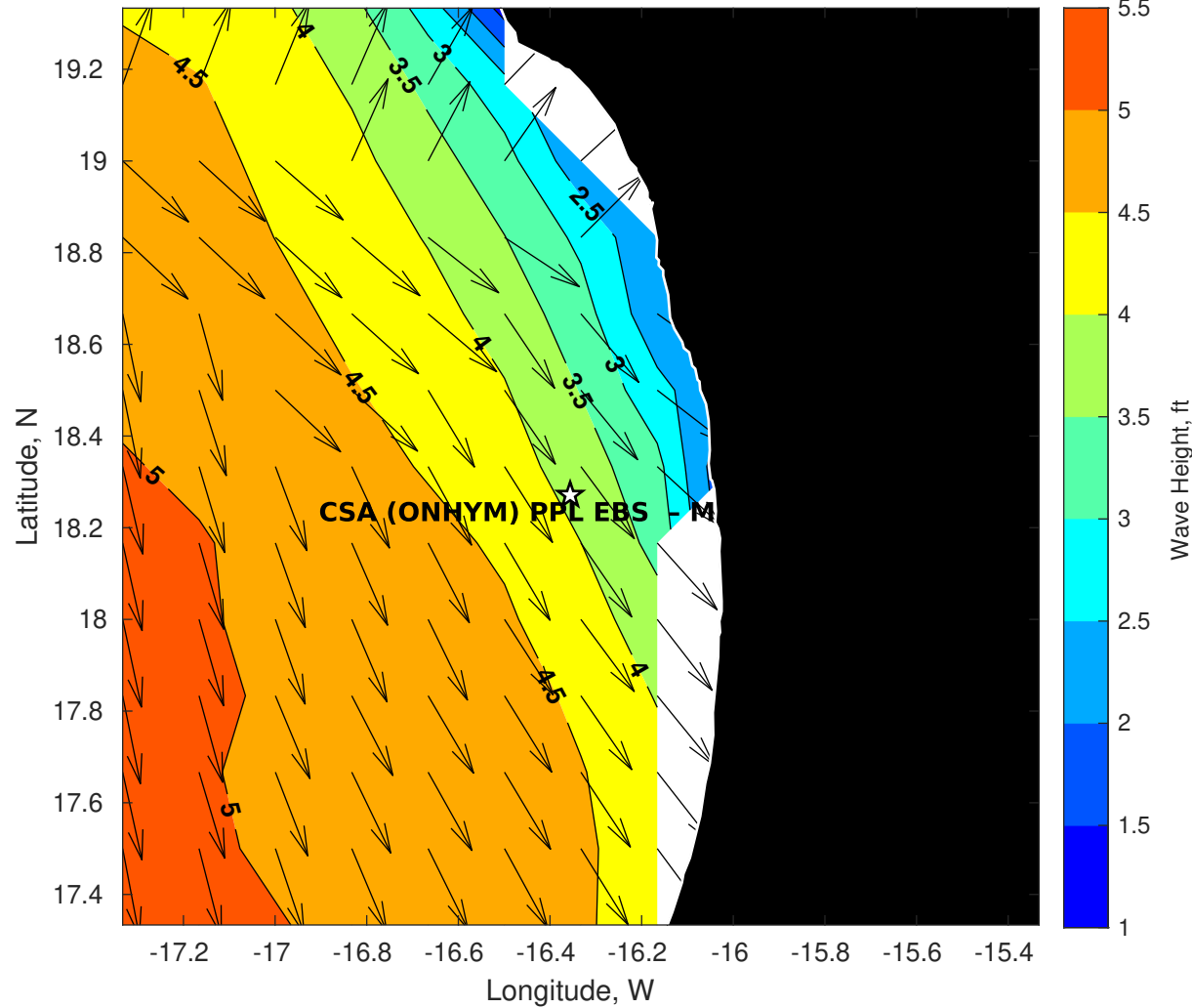
Wave Height (ft) for CSA (ONHYM) PPL EBS - Mauritania at 09-May-2025 09:00:00
