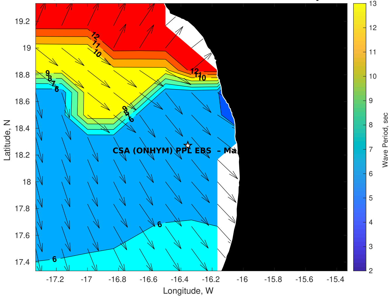
Wave Period (sec) for CSA (ONHYM) PPL EBS - Mauritania at 09-May-2025 09:00:00
