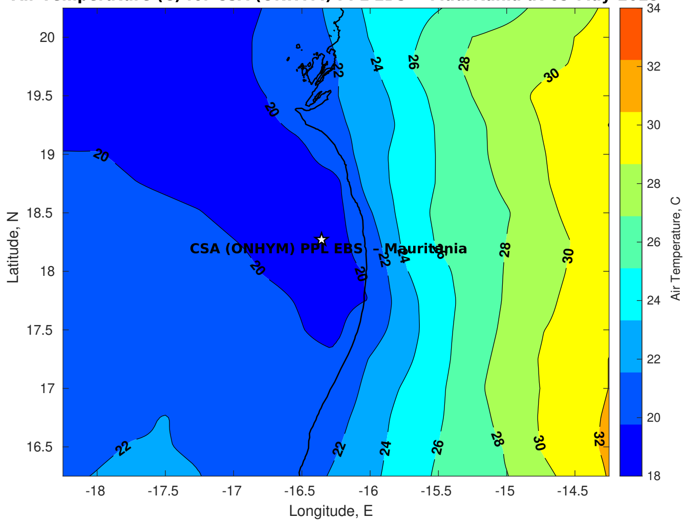
Air Temperature (C) for CSA (ONHYM) PPL EBS - Mauritania at 09-May-2025
