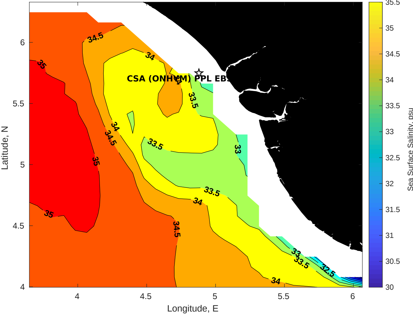
Surface Salinity for CSA (ONHYM) PPL EBS - Nigeria at 08-May-2025 00:00:00
