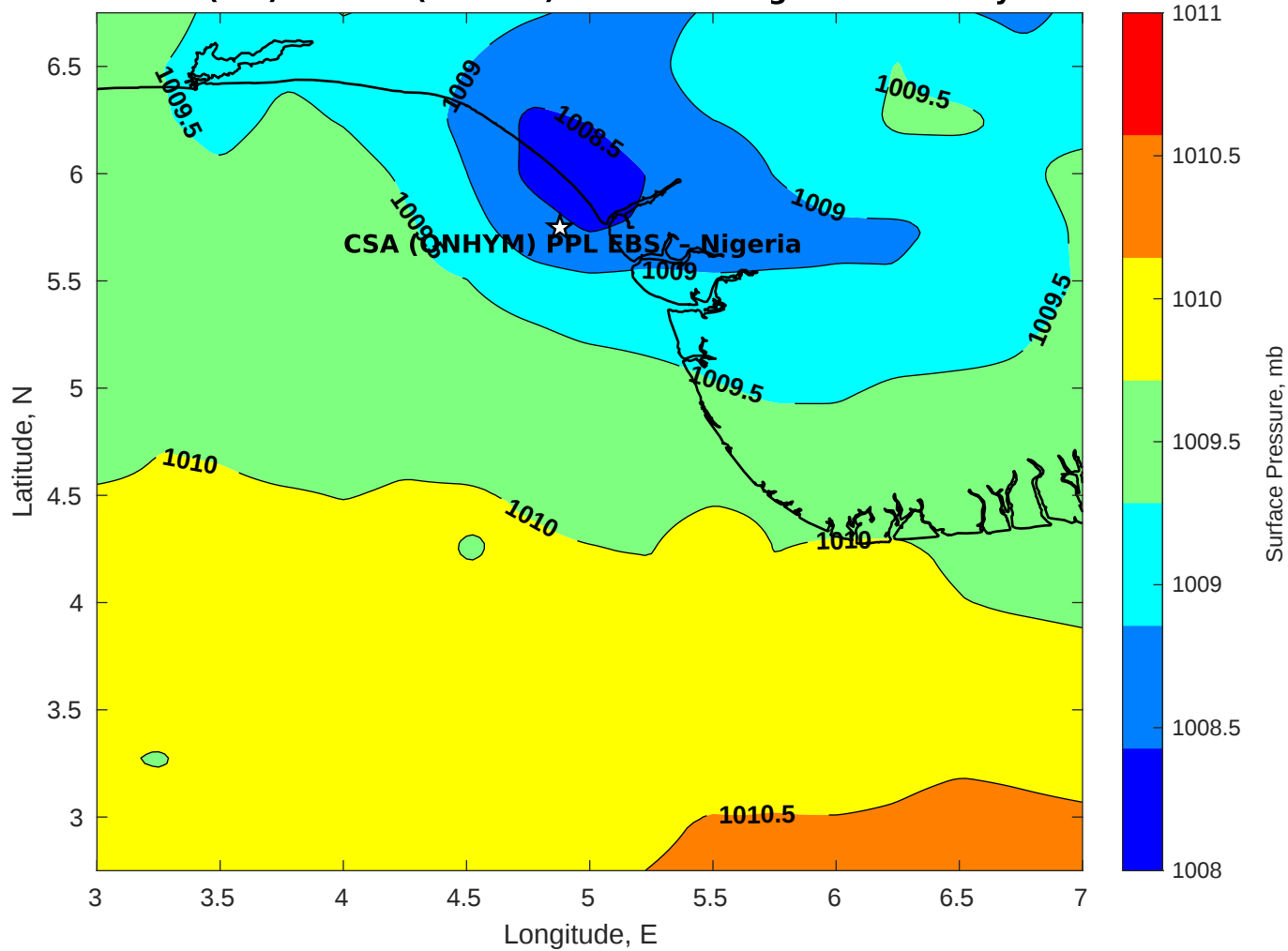
Surface Pressure (mb) for CSA (ONHYM) PPL EBS - Nigeria at 09-May-2025 00:00:00
