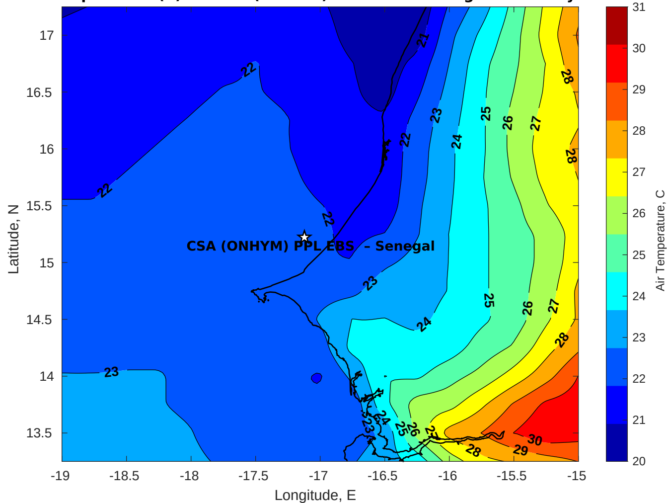
Air Temperature (C) for CSA (ONHYM) PPL EBS - Senegal at 09-May-2025
