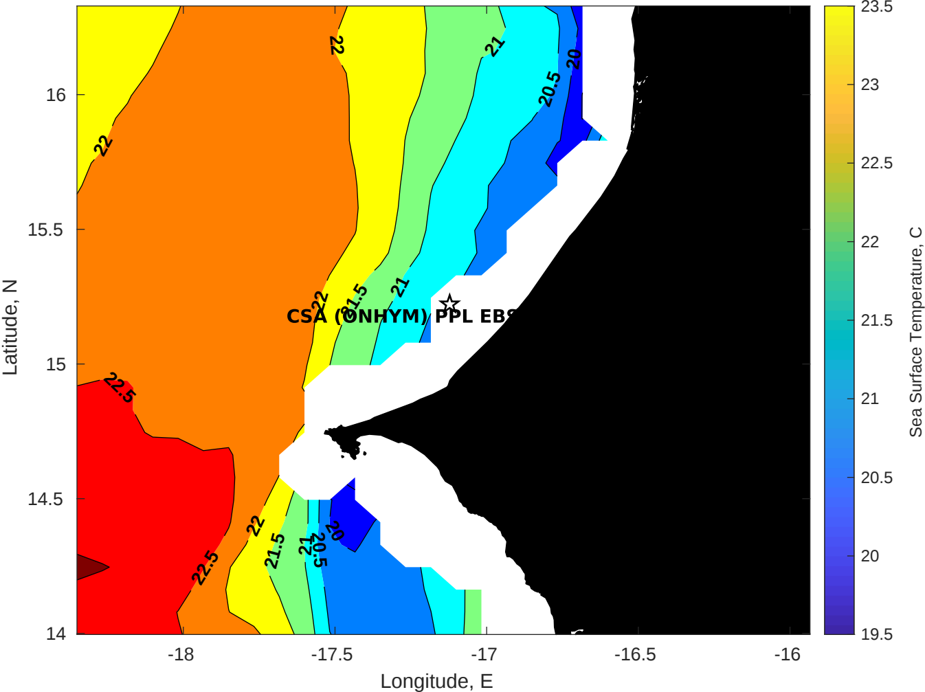
SST for CSA (ONHYM) PPL EBS - Senegal at 08-May-2025 00:00:00
