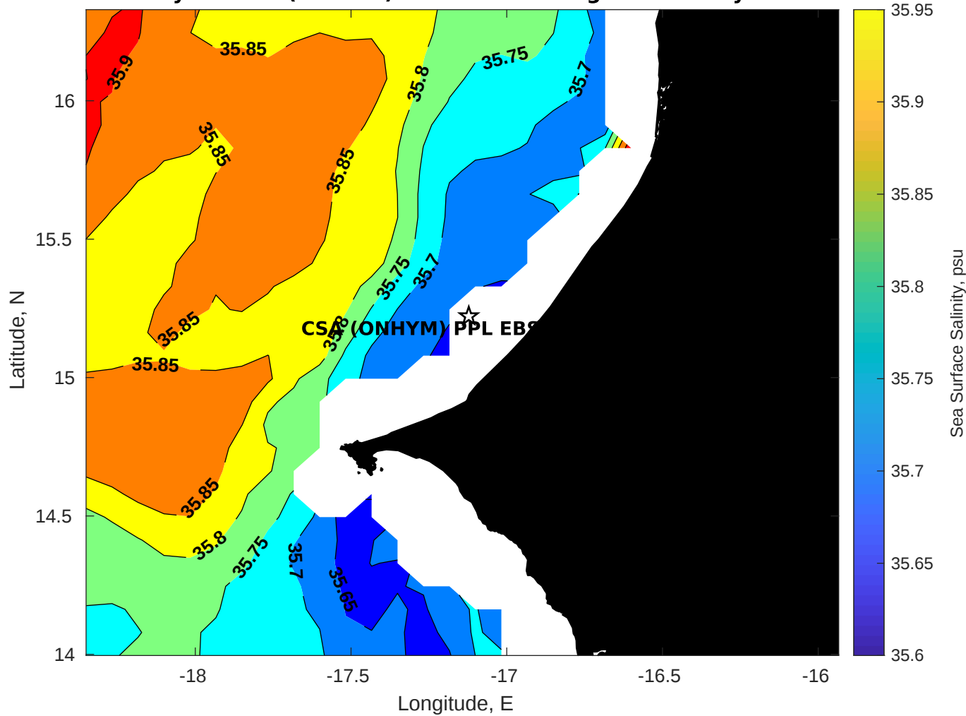
Surface Salinity for CSA (ONHYM) PPL EBS - Senegal at 08-May-2025 00:00:00
