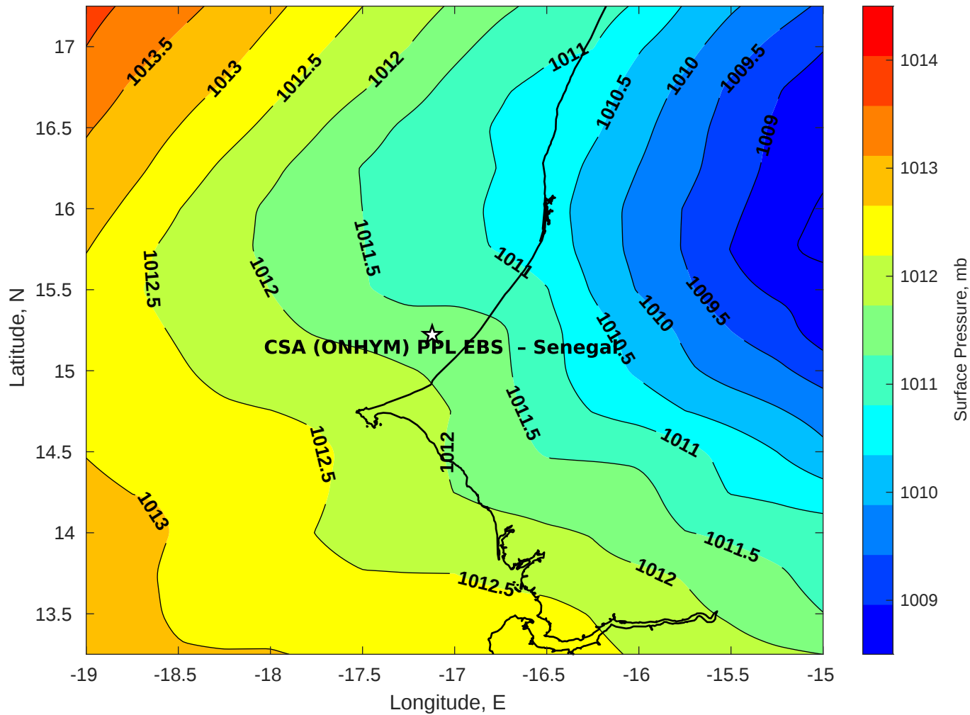
Surface Pressure (mb) for CSA (ONHYM) PPL EBS - Senegal at 09-May-2025 00:00:00
