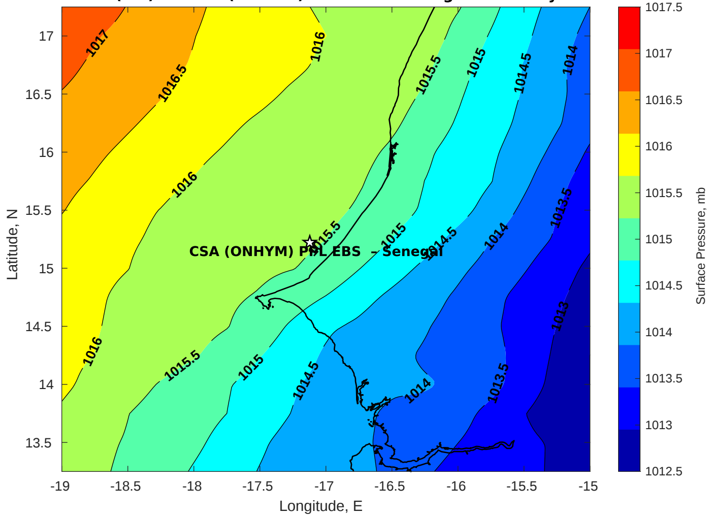
Surface Pressure (mb) for CSA (ONHYM) PPL EBS - Senegal at 11-May-2025 00:00:00
