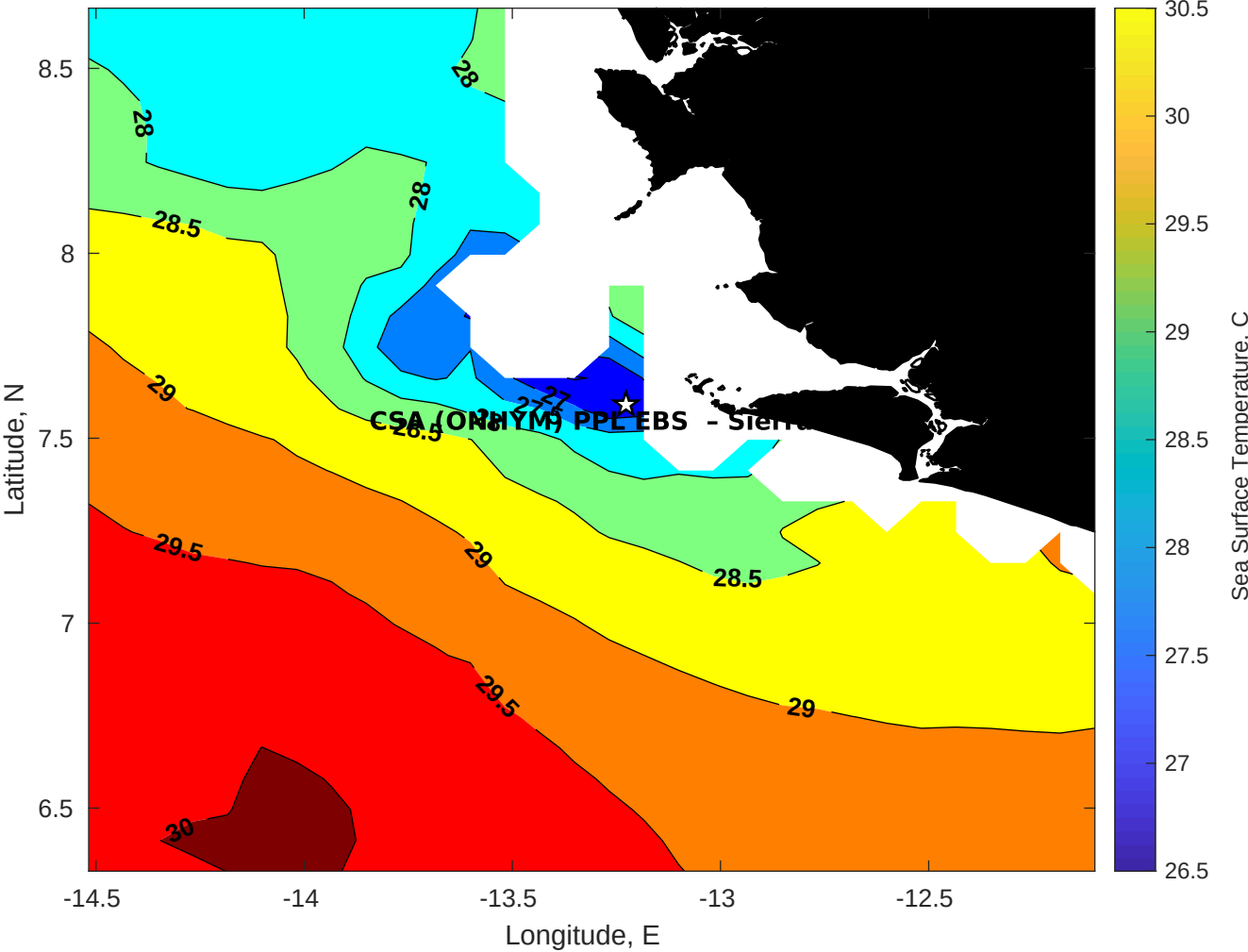
SST for CSA (ONHYM) PPL EBS - Sierra Leone at 08-May-2025 00:00:00
