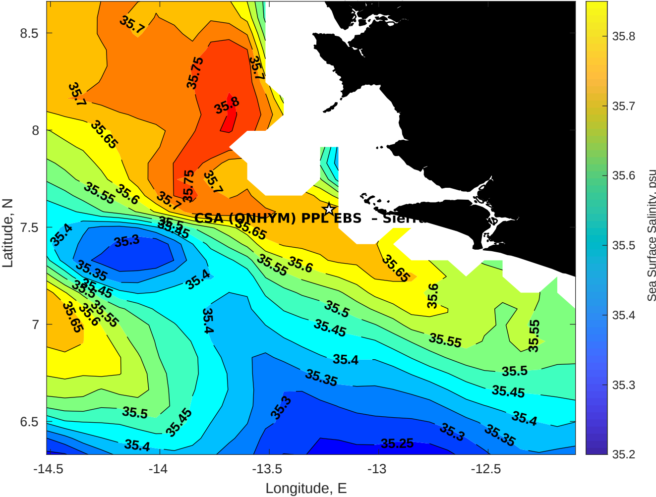
Surface Salinity for CSA (ONHYM) PPL EBS - Sierra Leone at 08-May-2025 00:00:00
