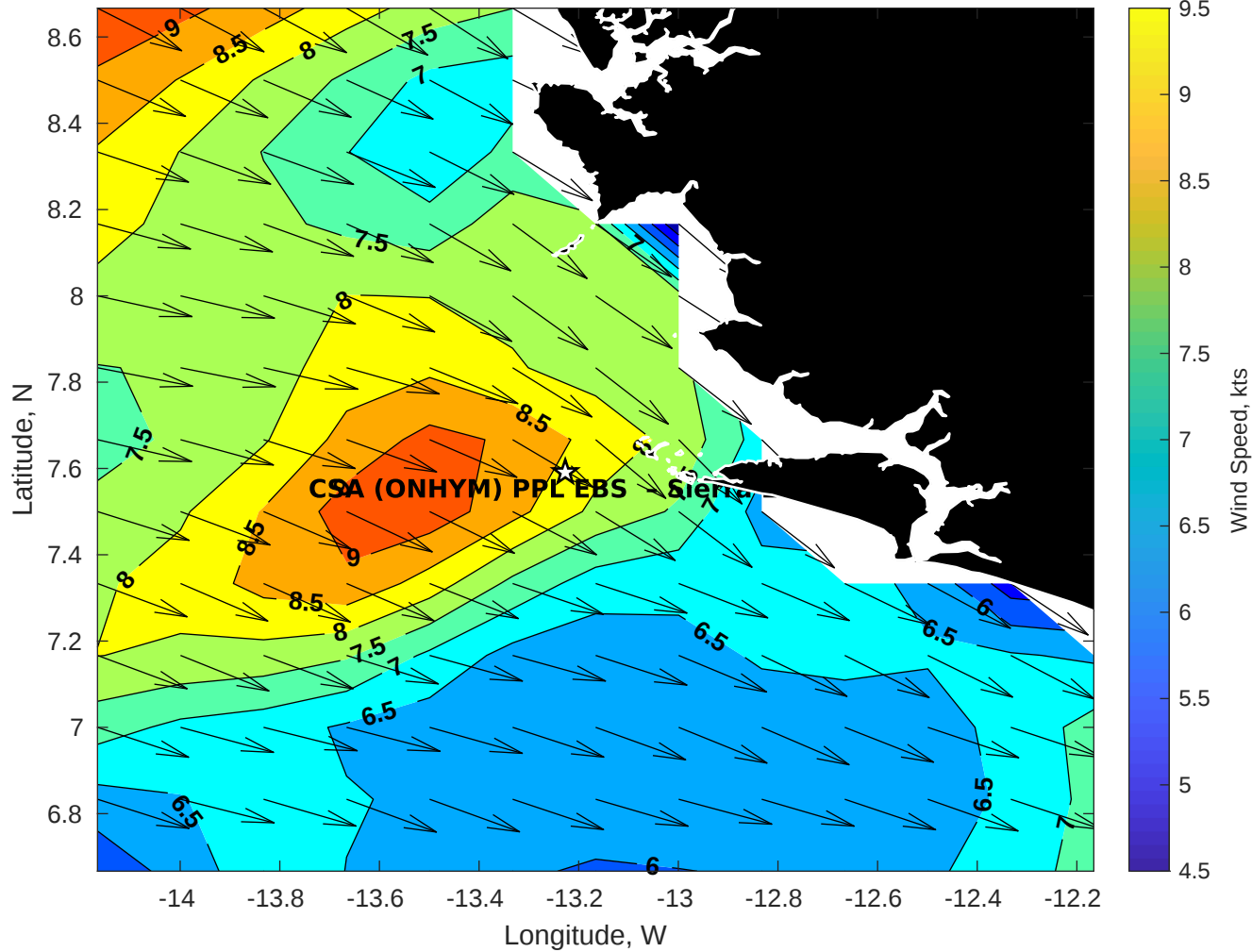
Winds (kts) for CSA (ONHYM) PPL EBS - Sierra Leone at 09-May-2025 09:00:00
