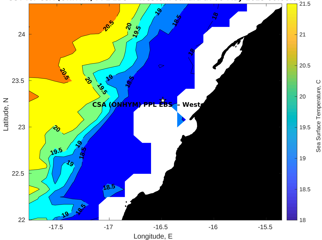
SST for CSA (ONHYM) PPL EBS - Western Sahara at 08-May-2025 00:00:00
