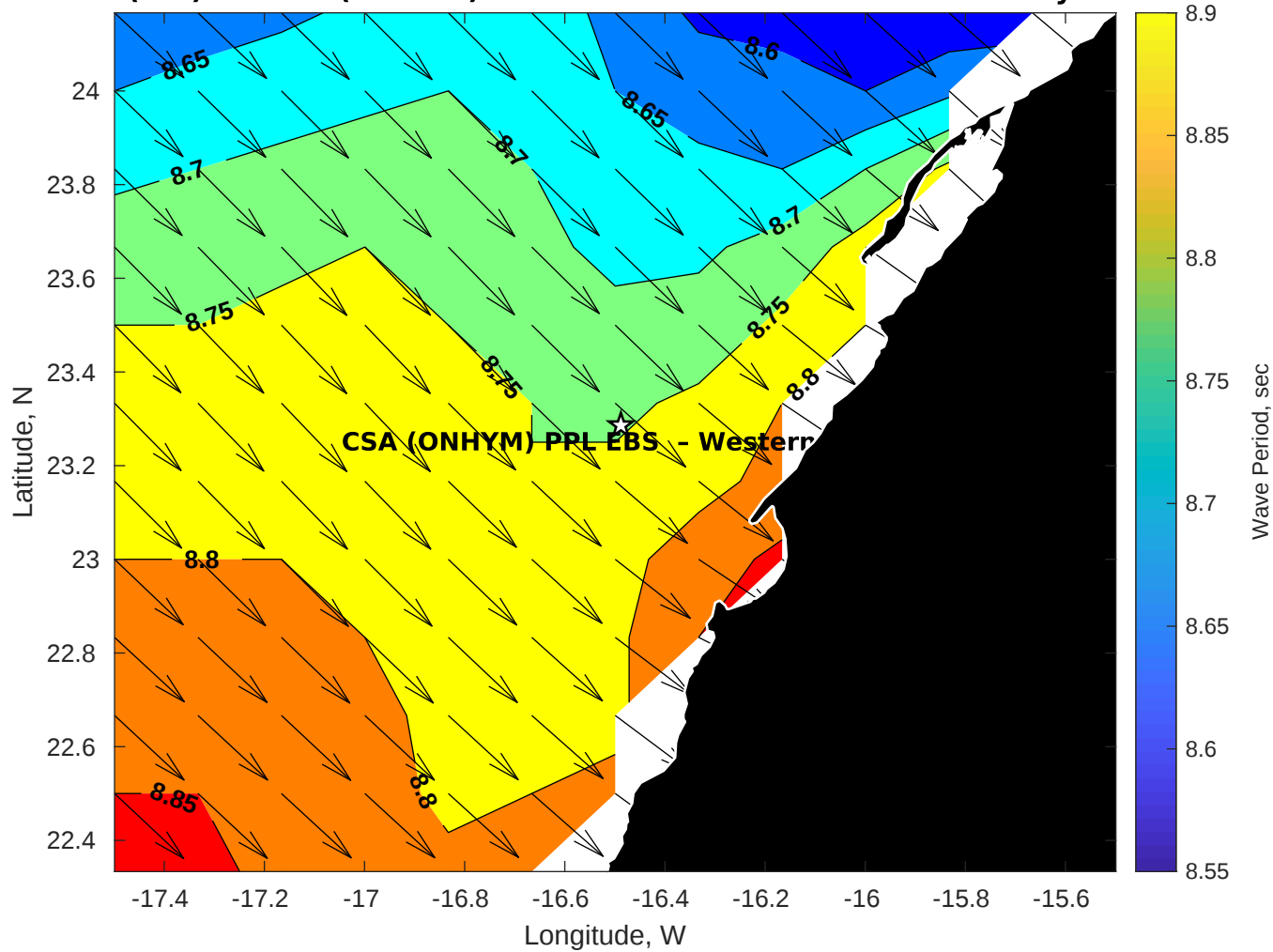
Wave Period (sec) for CSA (ONHYM) PPL EBS - Western Sahara at 09-May-2025 09:00:00
