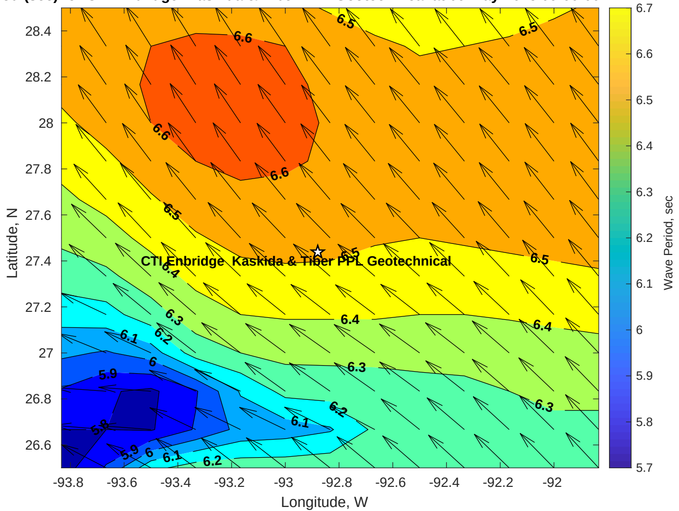
Wave Period (sec) for CTI Enbridge Kaskida & Tiber PPL Geotechnical at 09-May-2025 09:00:00
