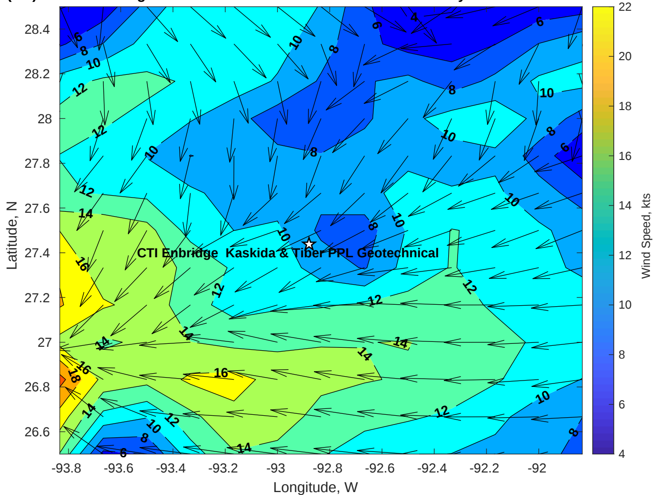
Winds (kts) for CTI Enbridge Kaskida & Tiber PPL Geotechnical at 09-May-2025 09:00:00
