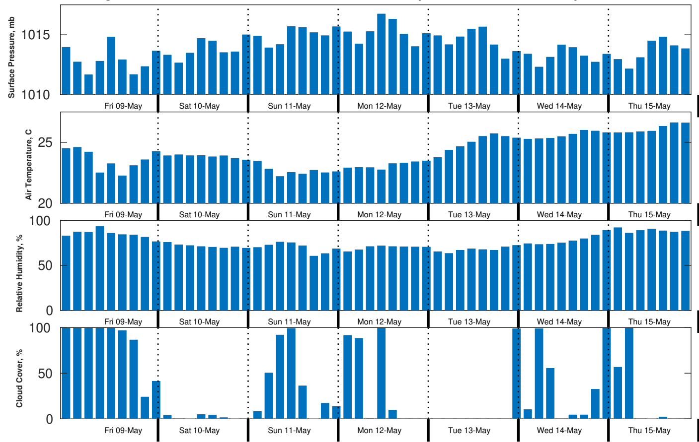
Met Forecast for CTI Enbridge Kaskida & Tiber PPL Geotechnical from 09-May-2025 00:00:00 to 16-May-2025 00:00:00
