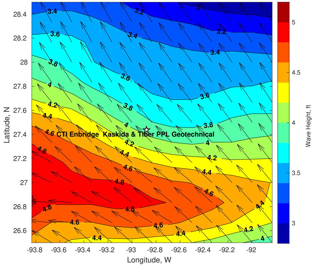
Wave Height (ft) for CTI Enbridge Kaskida & Tiber PPL Geotechnical at 09-May-2025 09:00:00
