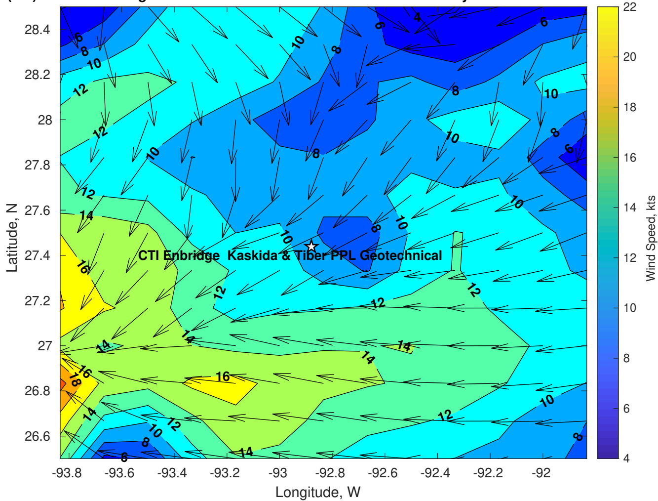
Winds (kts) for CTI Enbridge Kaskida & Tiber PPL Geotechnical at 09-May-2025 09:00:00
