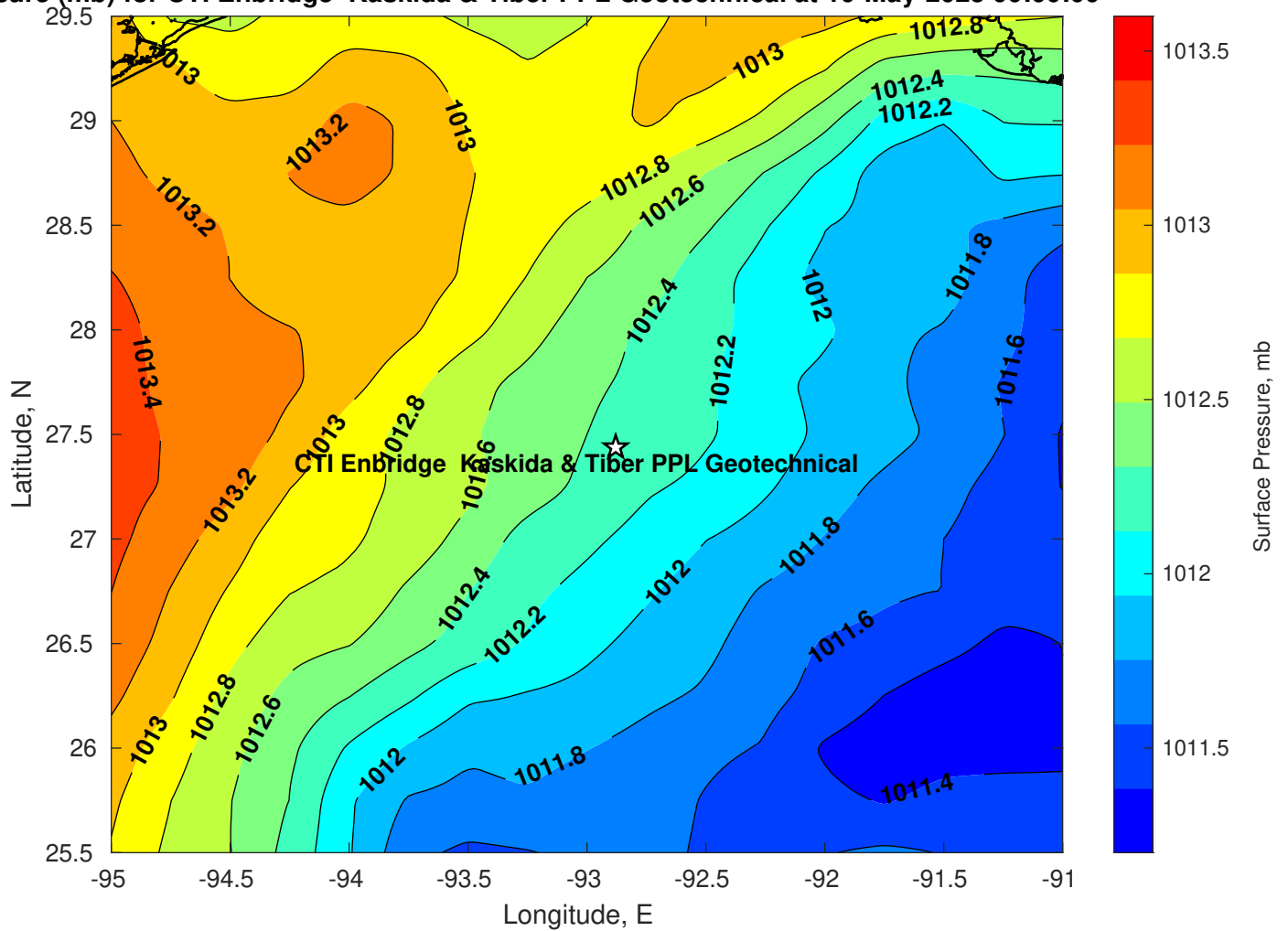
Surface Pressure (mb) for CTI Enbridge Kaskida & Tiber PPL Geotechnical at 10-May-2025 00:00:00
