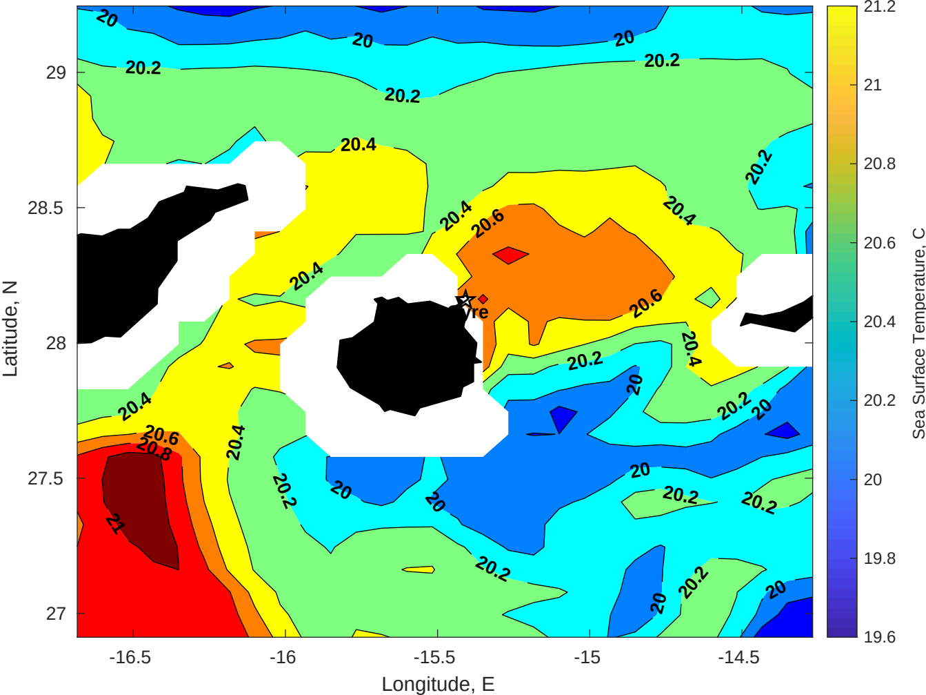
SST for Gyre at 08-May-2025 00:00:00
