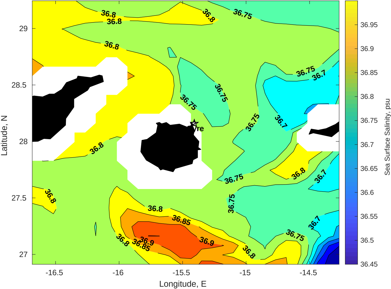
Surface Salinity for Gyre at 08-May-2025 00:00:00
