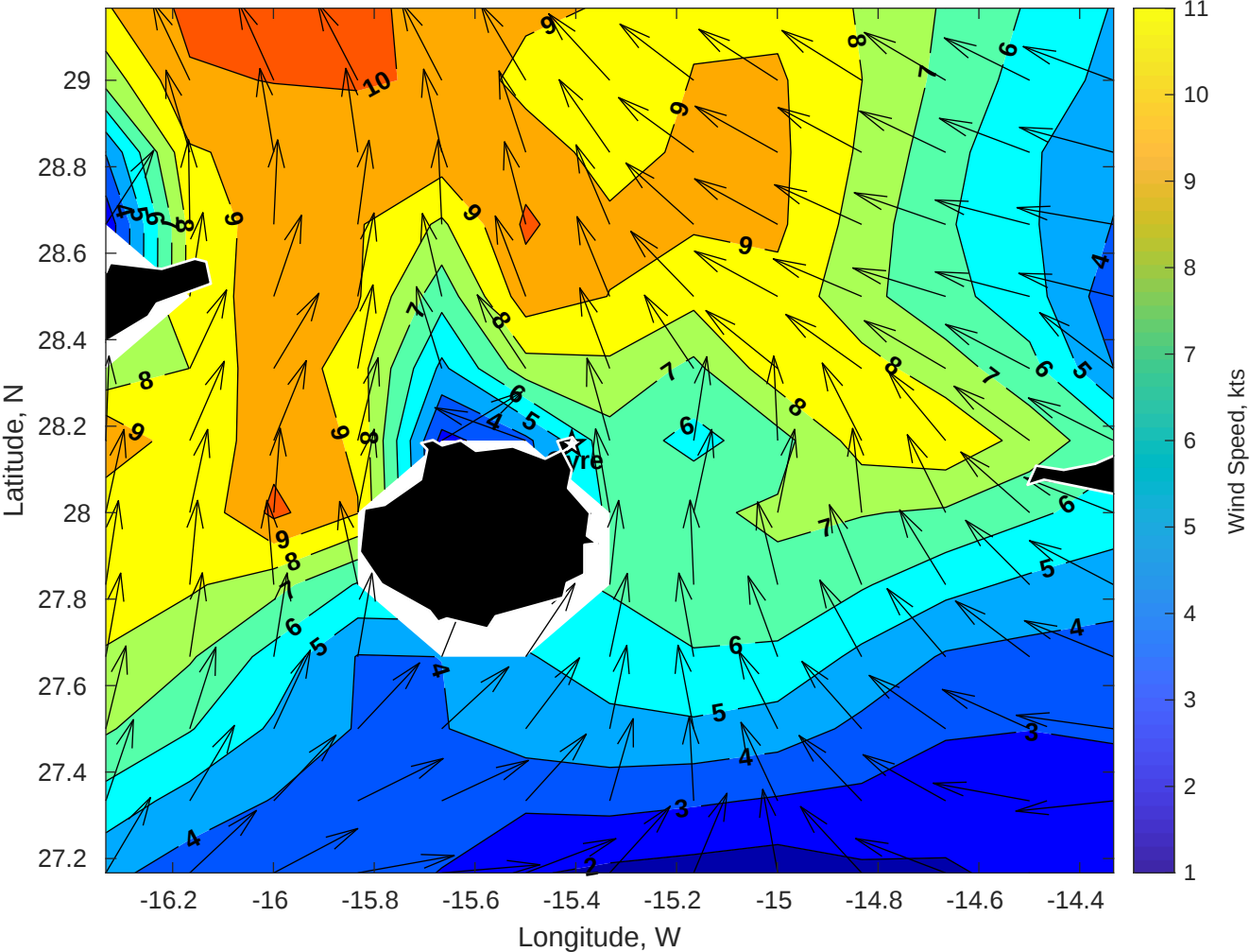
Winds (kts) for Gyre at 09-May-2025 09:00:00
