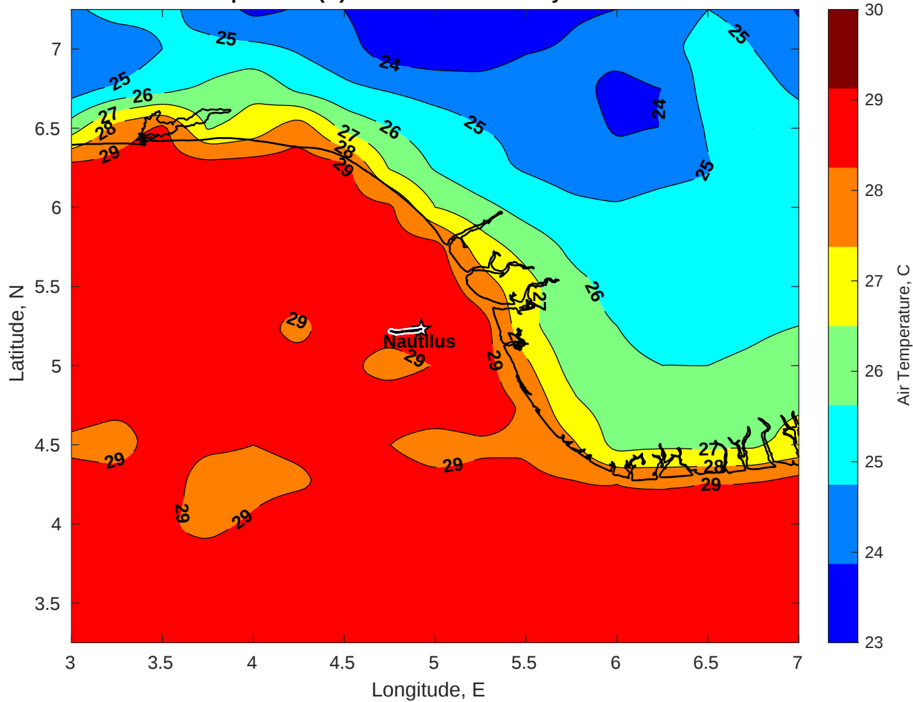
Air Temperature (C) for Nautilus at 09-May-2025
