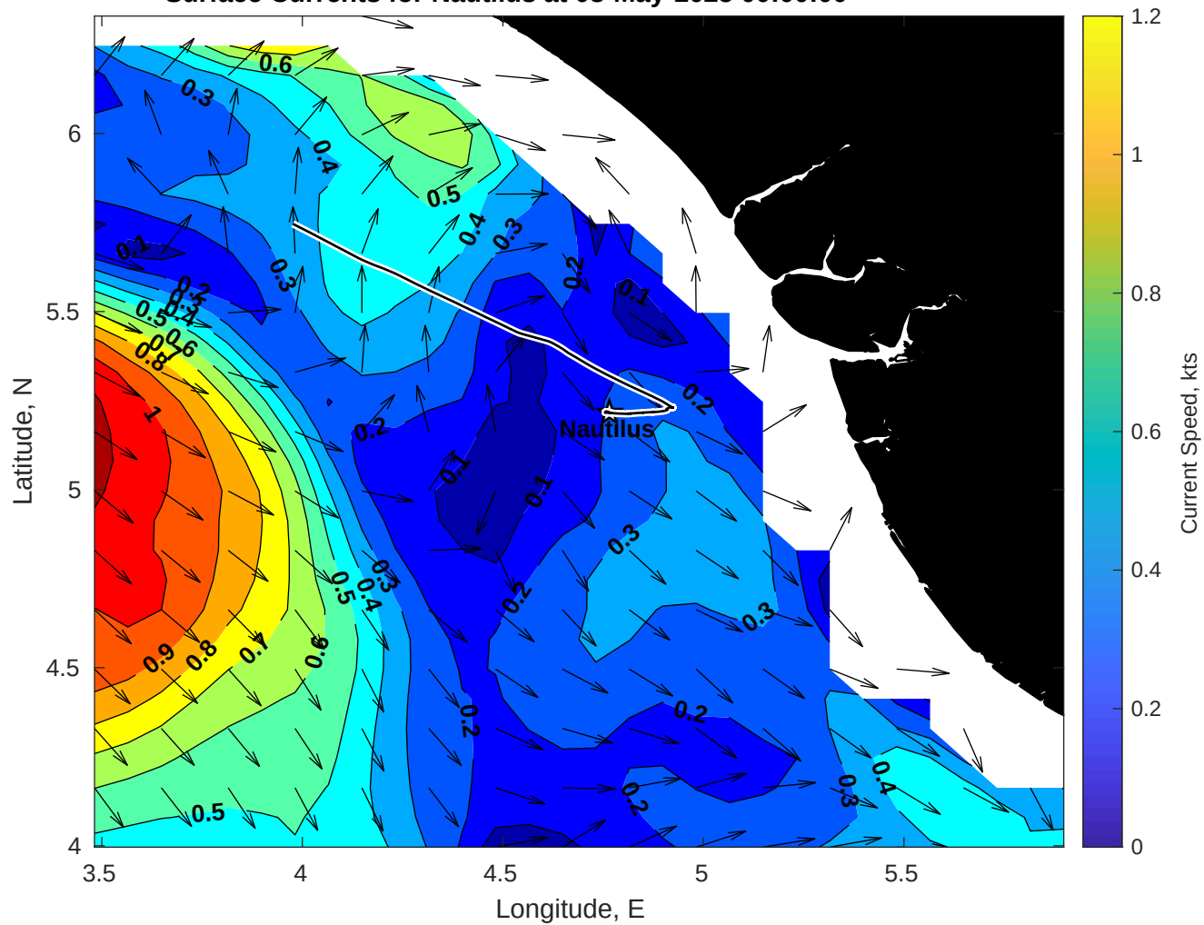
Surface Currents for Nautilus at 08-May-2025 00:00:00
