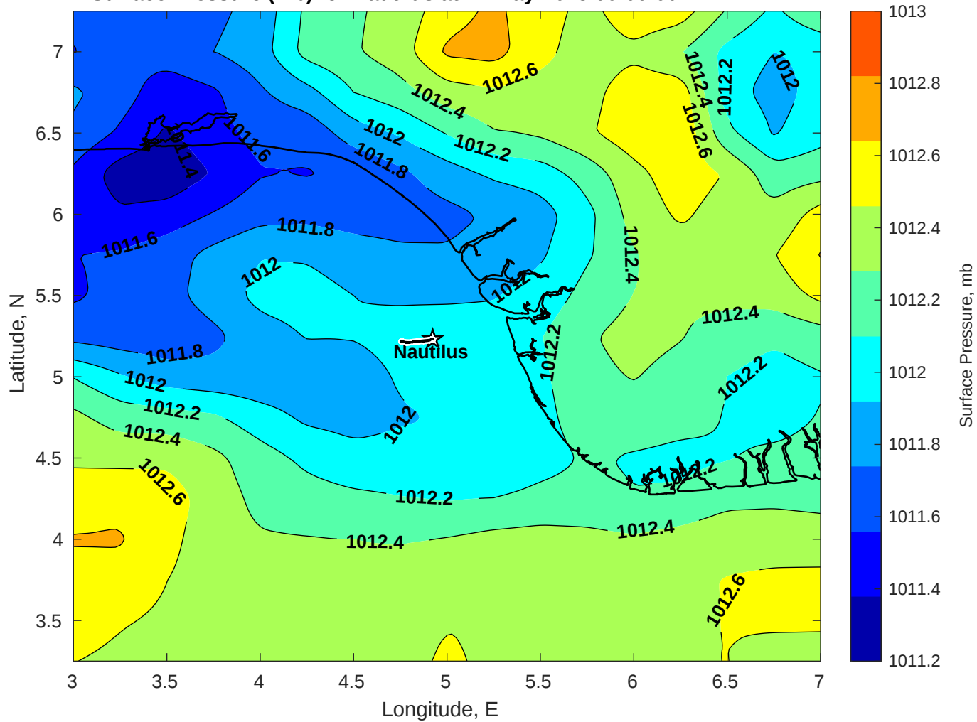
Surface Pressure (mb) for Nautilus at 11-May-2025 00:00:00
