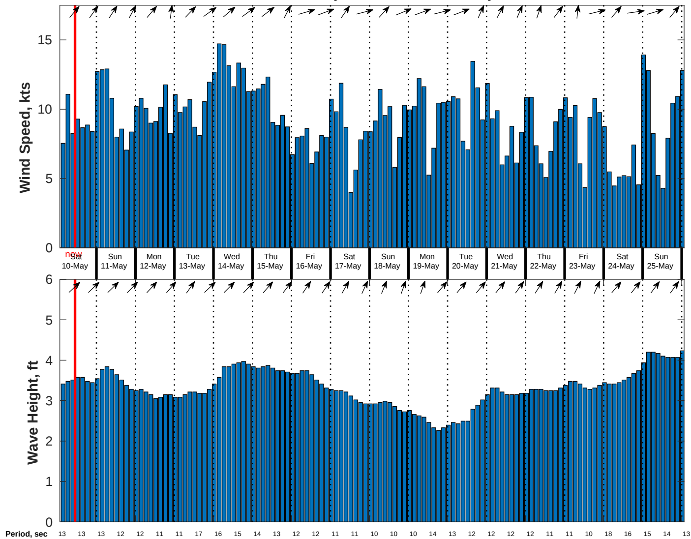
Wind & Wave Forecast for Nautilus from 09-May-2025 02:00:00 to 25-May-2025 02:00:00
