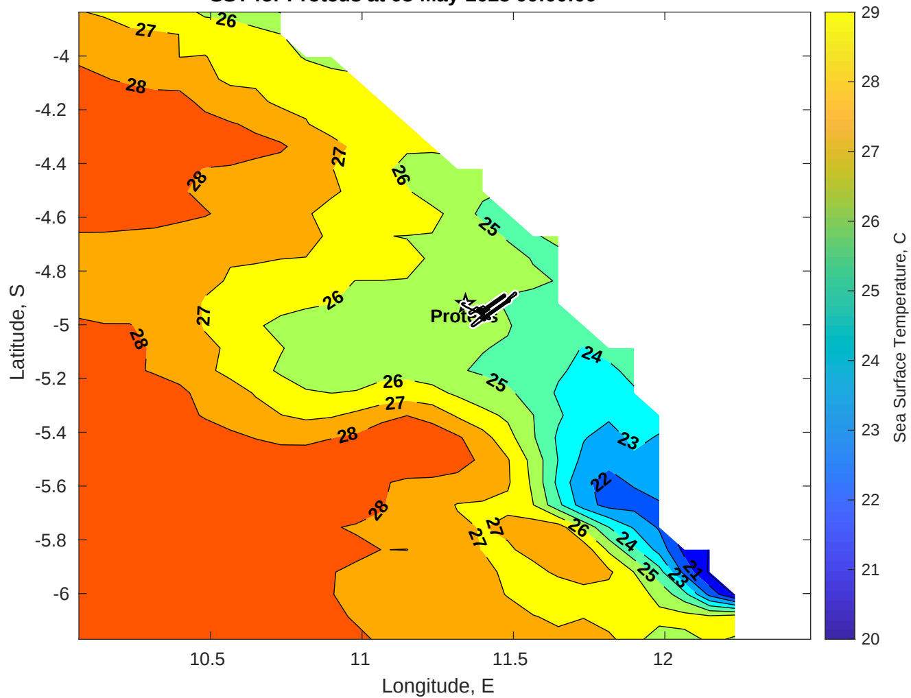
SST for Proteus at 08-May-2025 00:00:00
