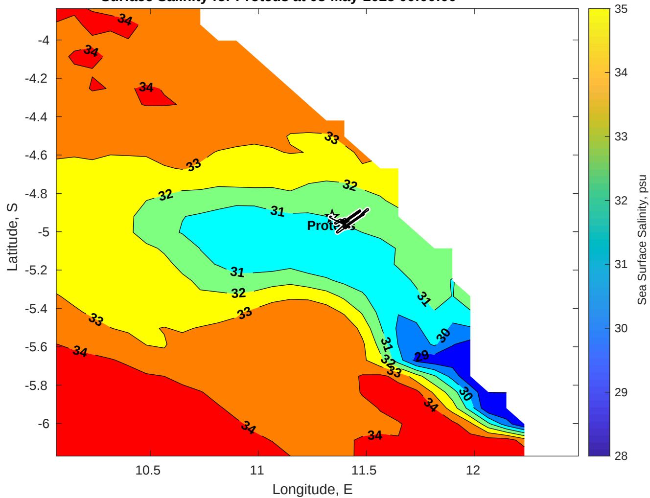
Surface Salinity for Proteus at 08-May-2025 00:00:00
