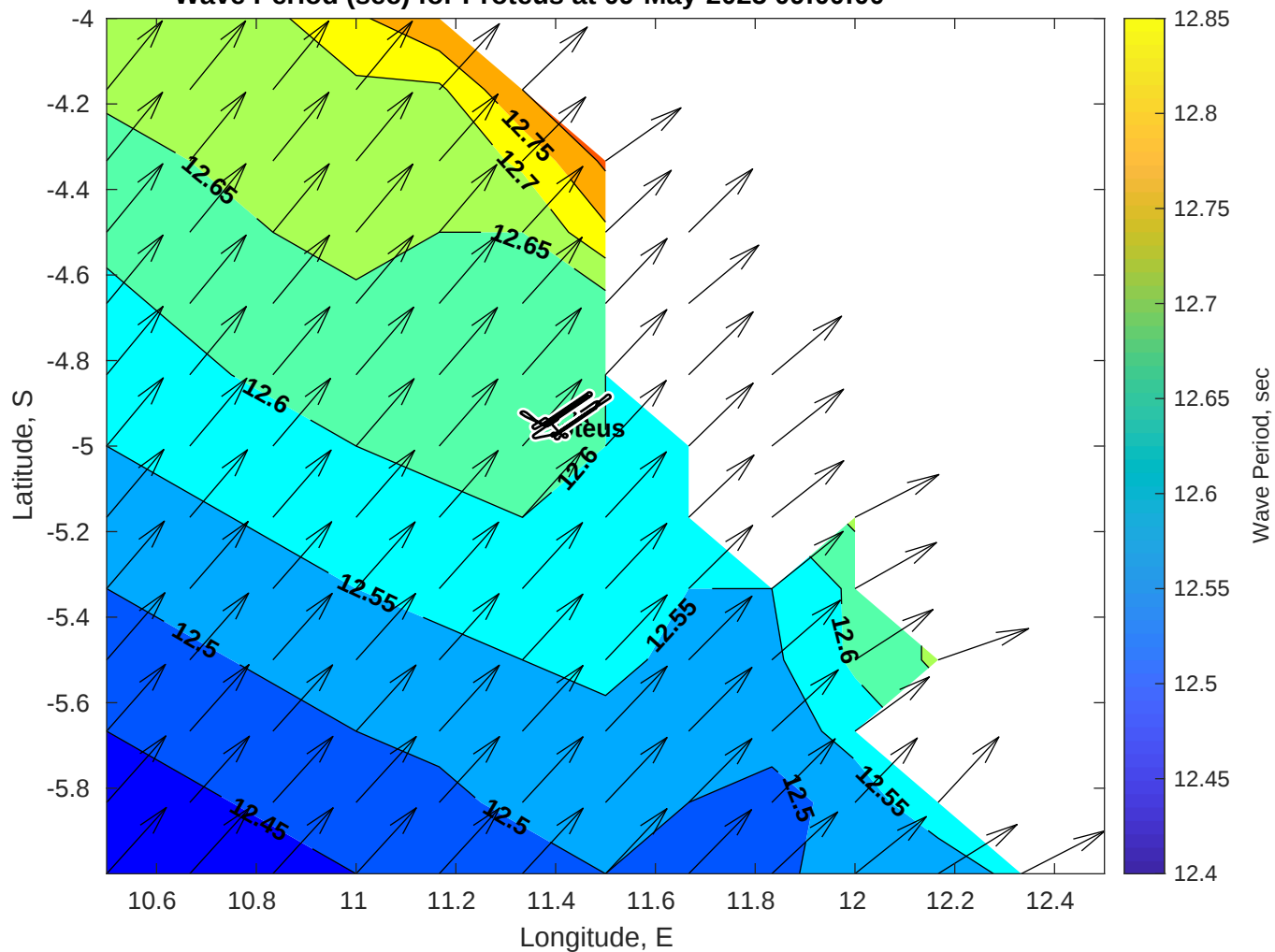
Wave Period (sec) for Proteus at 09-May-2025 09:00:00
