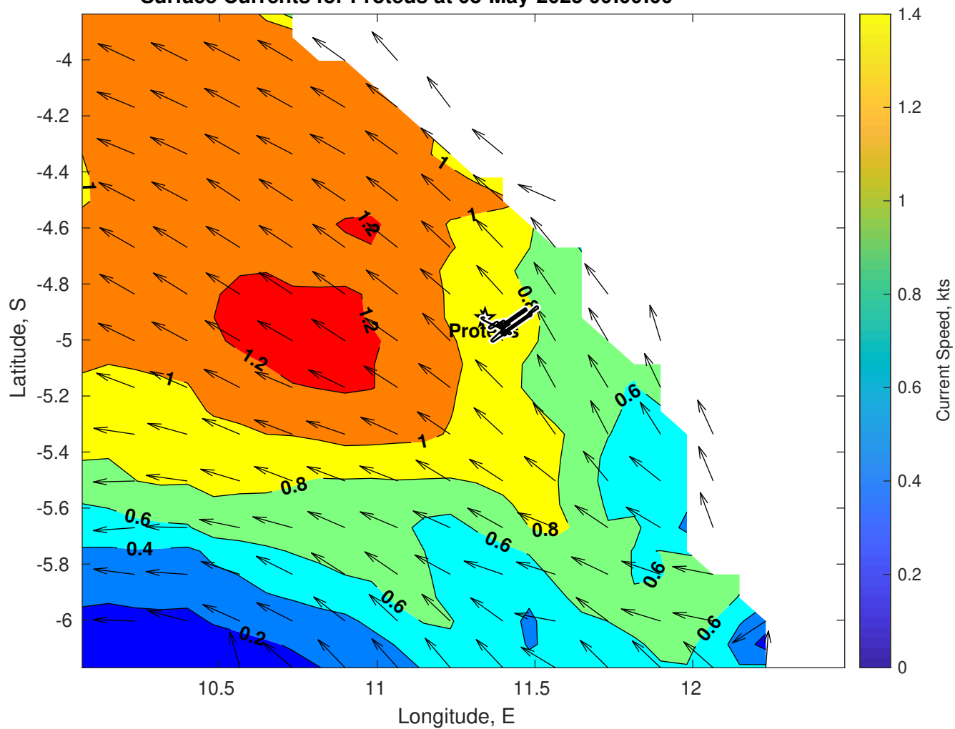
Surface Currents for Proteus at 08-May-2025 00:00:00
