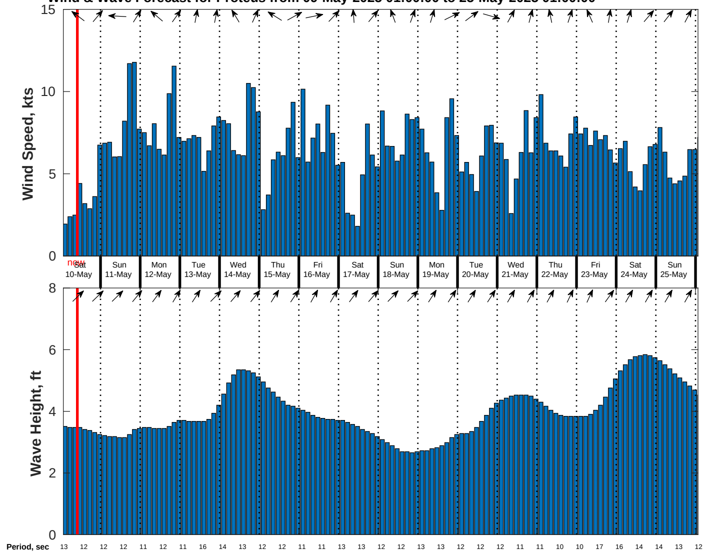
Wind & Wave Forecast for Proteus from 09-May-2025 01:00:00 to 25-May-2025 01:00:00
