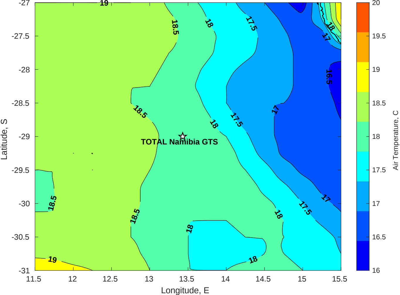
Air Temperature (C) for TOTAL Namibia GTS at 09-May-2025
