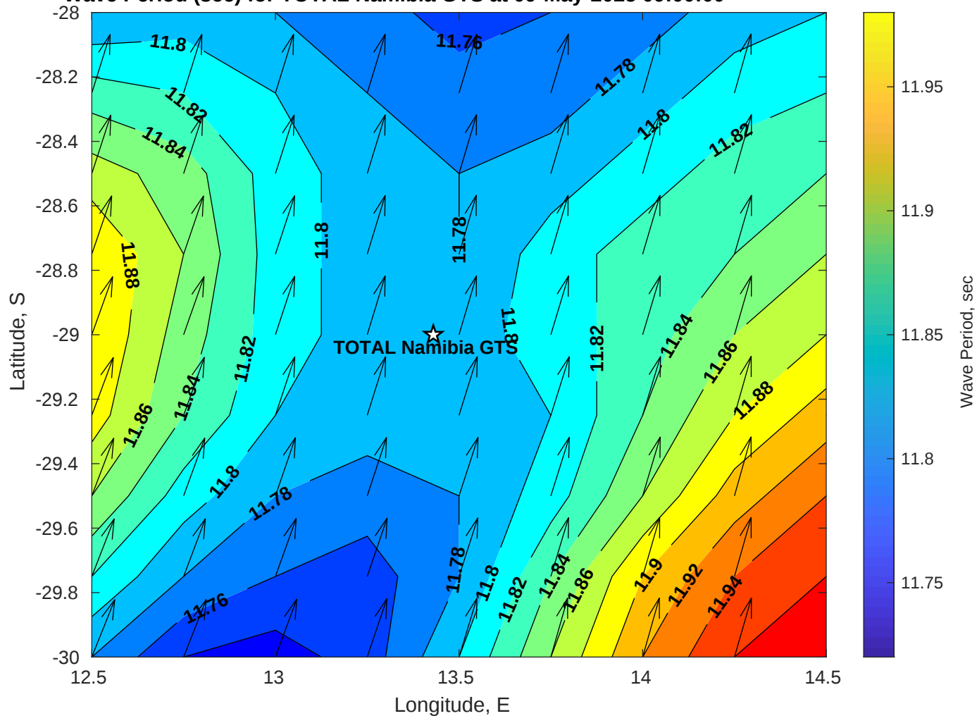
Wave Period (sec) for TOTAL Namibia GTS at 09-May-2025 09:00:00
