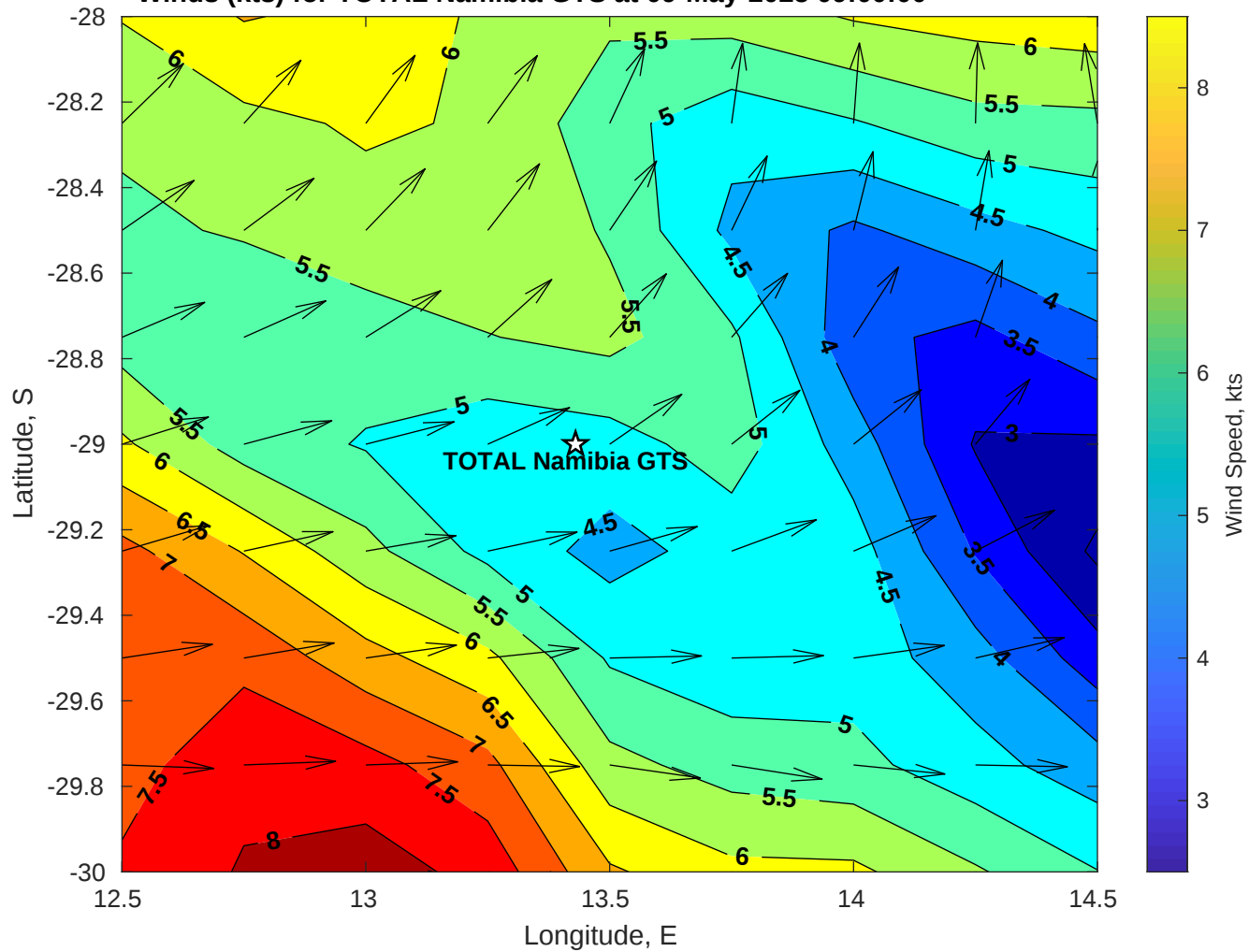
Winds (kts) for TOTAL Namibia GTS at 09-May-2025 09:00:00
