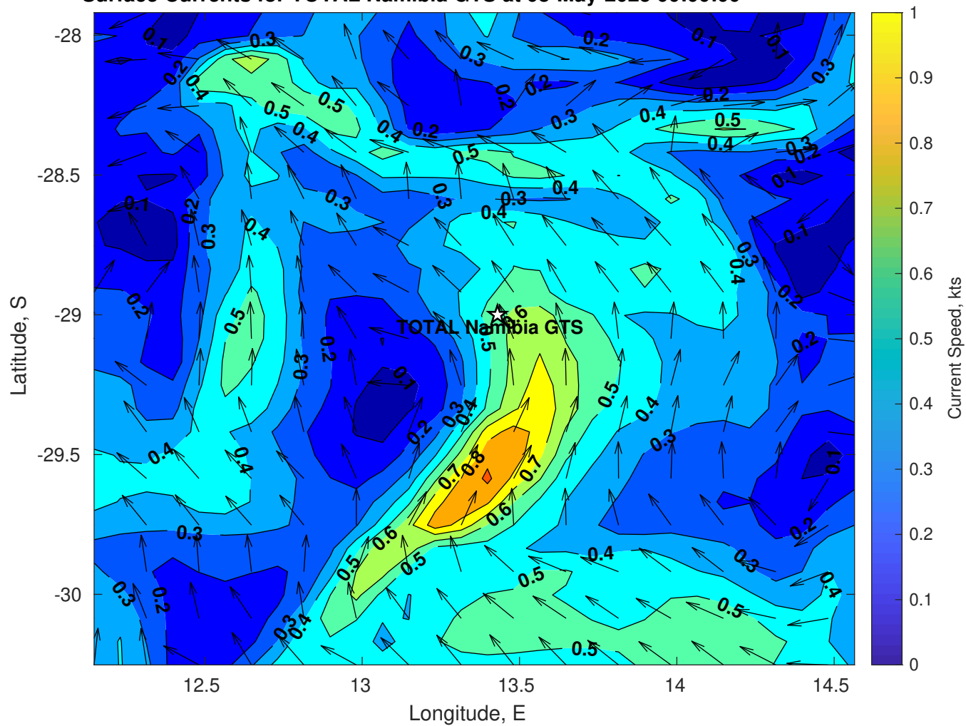
Surface Currents for TOTAL Namibia GTS at 08-May-2025 00:00:00
