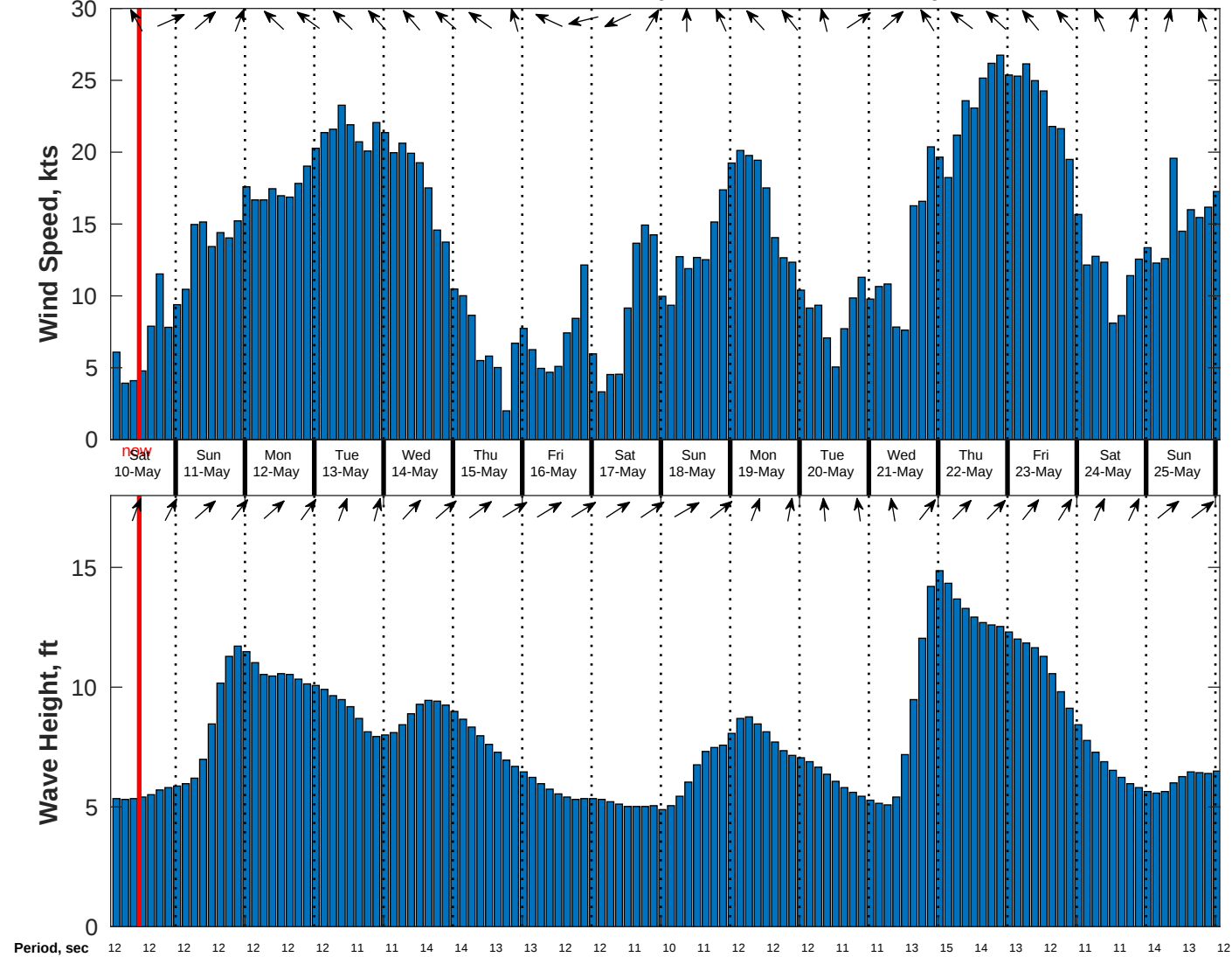
Wind & Wave Forecast for TOTAL Namibia GTS from 09-May-2025 02:00:00 to 25-May-2025 02:00:00
