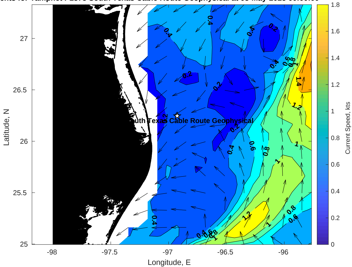
Surface Currents for Tampnet P2378 South Texas Cable Route Geophysical at 08-May-2025 00:00:00
