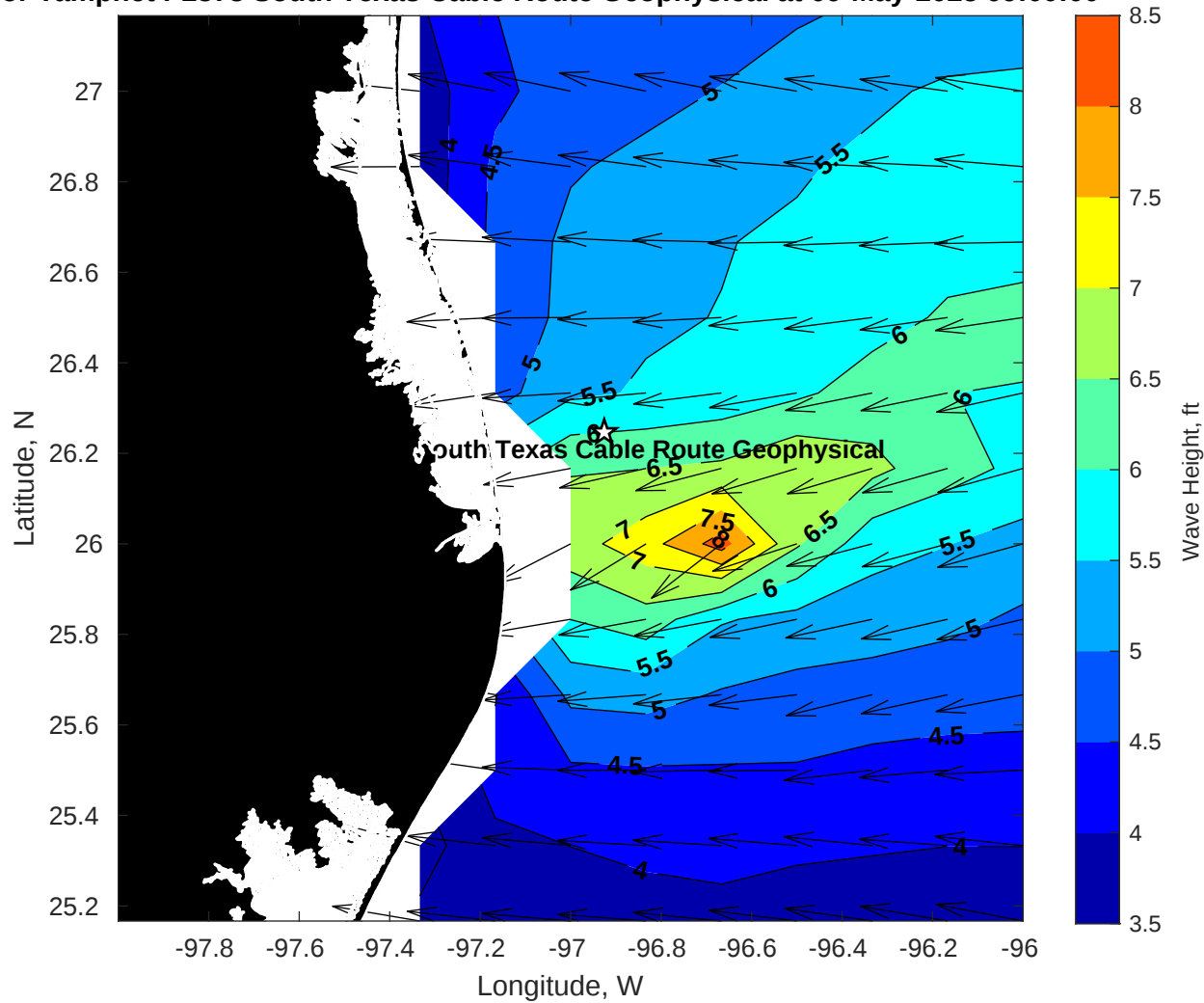
Wave Height (ft) for Tampnet P2378 South Texas Cable Route Geophysical at 09-May-2025 09:00:00
